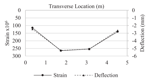
Figure 9 Load Case 2 Strain and Deflection – 4-Girders
