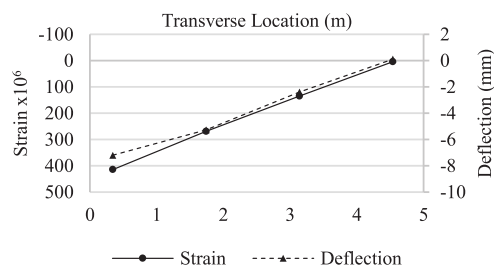
Figure 8 Load Case 1 Strain and Deflection – 4-Girders
