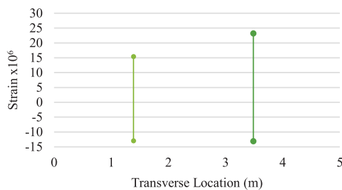
Figure 22 Deck Strain at Maximum Load – Load Case 3, 3-Girders
