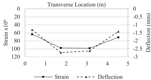
Figure 11 Load Case 4 Strain and Deflection – 4-Girders
