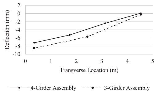
Figure 24 Deflection Comparison for Load Case 1
