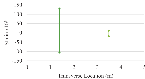
Figure 20 Deck Strain at Maximum Load – Load Case 1, 3-Girders
