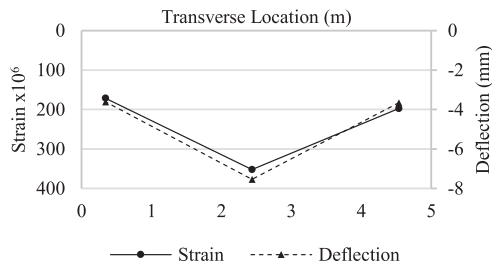
Figure 17 Load Case 2 Strain and Deflection – 3-Girders
