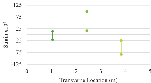
Figure 12 CLT Deck Strain at Maximum Load – Load Case 1, 4-Girders
