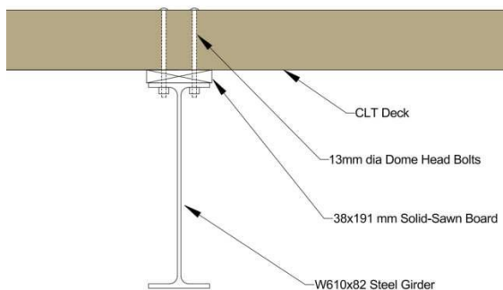
Figure 3 CLT Panel Connection to Girder
