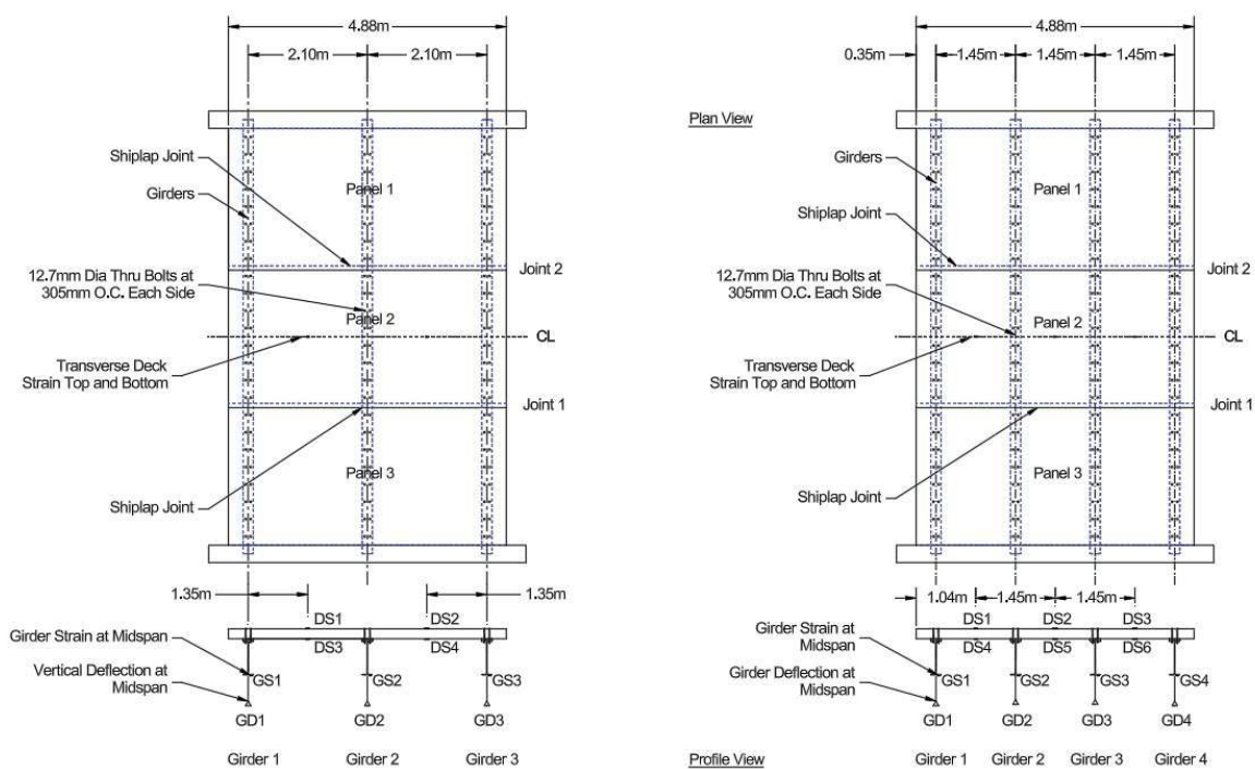
Figure 6 Transverse deck panel and instrumentation configuration for 3- and 4-girder assemblies
