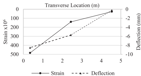
Figure 16 Load Case 1 Strain and Deflection – 3-Girders
