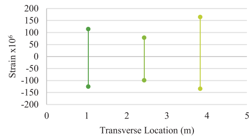
Figure 13 Deck Strain at Maximum Load – Load Case 2, 4-Girders
