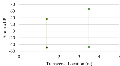
Figure 23 Deck Strain at Maximum Load – Load Case 4, 3-Girders
