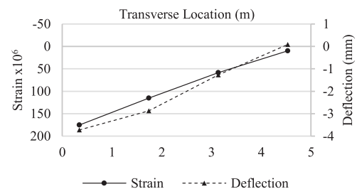
Figure 10 Load Case 3 Strain and Deflection – 4-Girders
