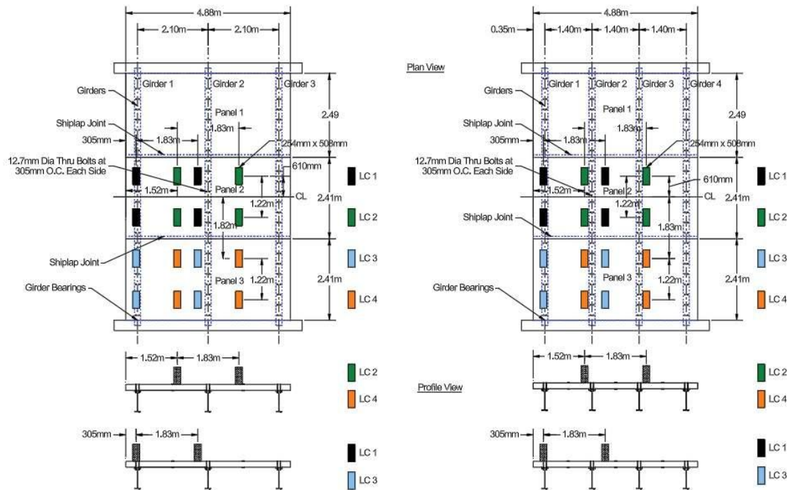
Figure 7 Location of rear-axle tandems for each load case for 3- and 4-girder assemblies
