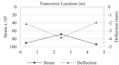
Figure 19 Load Case 4 Strain and Deflection – 3-Girders
