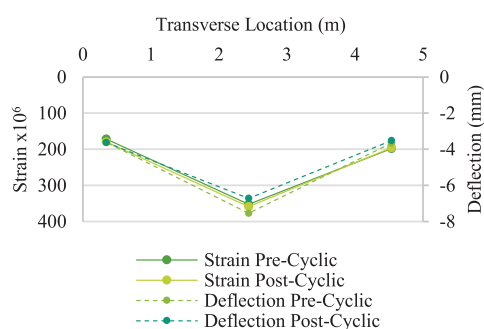
Figure 26 Load Case 2 Strain and Deflection – 3 Girders, Pre- and Post-Cyclic Loading
