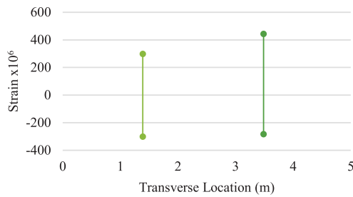
Figure 21 Deck Strain at Maximum Load – Load Case 2, 3-Girders
