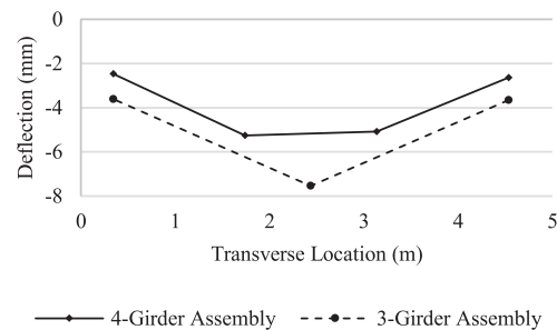
Figure 25 Deflection Comparison for Load Case 2
