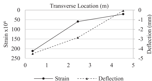
Figure 18 Load Case 3 Strain and Deflection – 3-Girders
