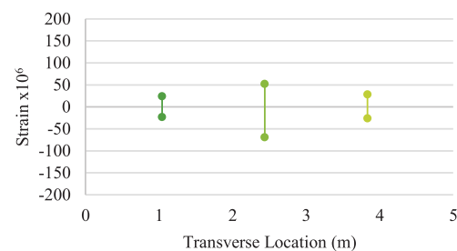
Figure 15 Deck Strain at Maximum Load – Load Case 4, 4-Girders
