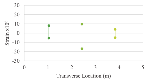
Figure 14 Deck Strain at Maximum Load – Load Case 3, 4-Girders
