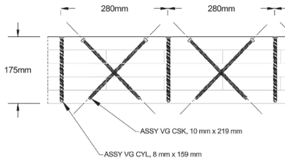
Figure 2 Half-Lap Joint Screw Pattern
