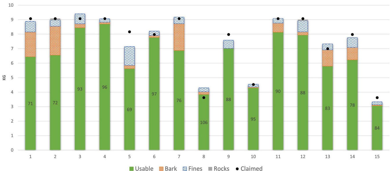
Figure 9.—Analysis of the weight of charcoal and extraneous materials per bag. The figure shows the proportion of charcoal fragments over 1/2 inch (noted as usable), bark, fines, and rocks (from bottom to top, respectively) in each bag. The black circles represent the claimed weight, while the total bar length represents the measured weight. Percentages (numeric values reported in the green bars) of usable charcoal fragments over 1/2 inch are calculated based on the claimed weight.
