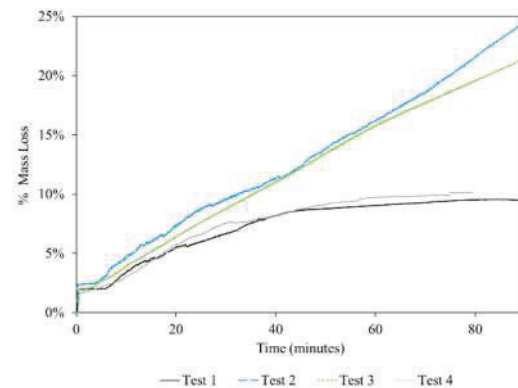
Figure 10: Percent mass loss curves from WOODWISE tests 1 - 4.
