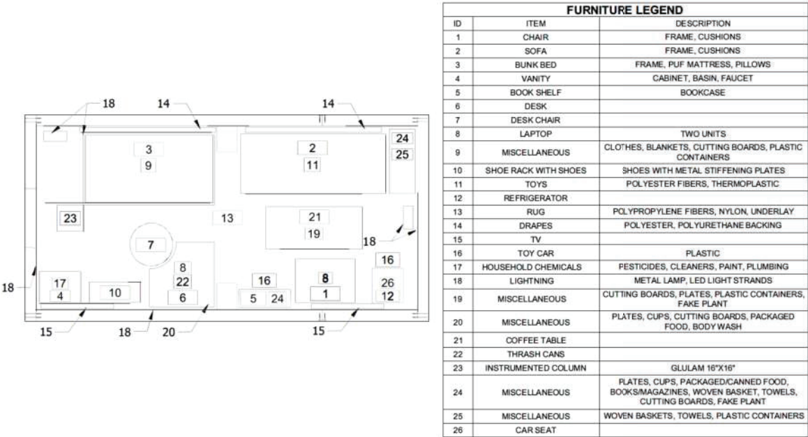
Figure 4: Schematic of modern fuel load layout for Tests #1 through #3.
