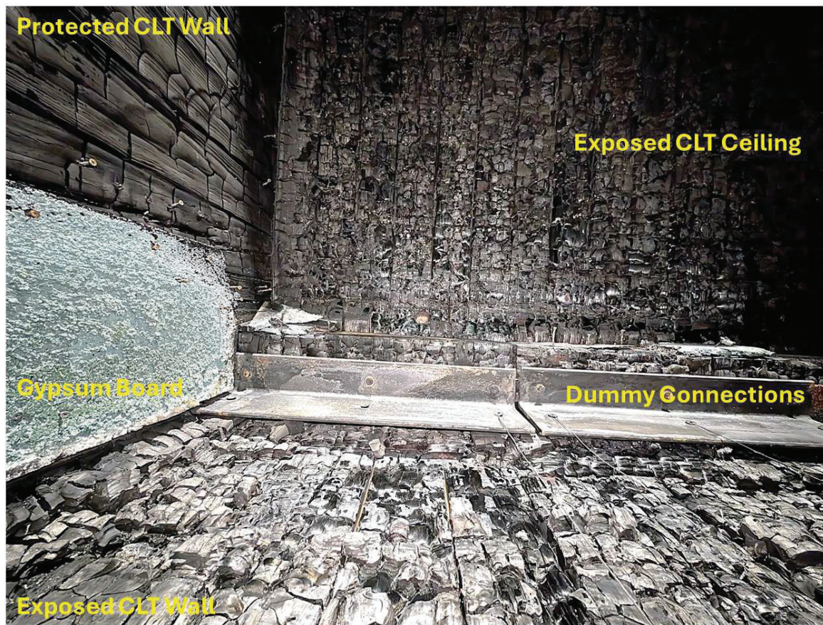
Figure 11: Charring patterns from different surfaces in Test 3.
