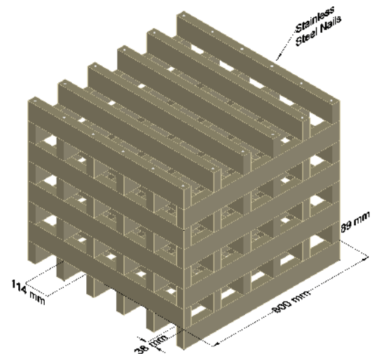
Figure 5: Schematic of wood cribs.
