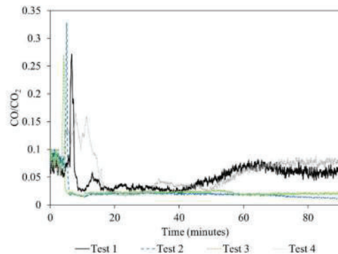
Figure 9: CO/CO 2 curves from WOODWISE Tests #1 through #4.
