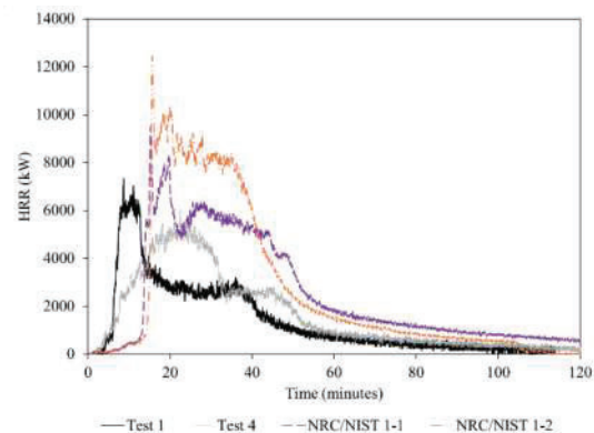
Figure 8: Heat release rate curves from WOODWISE Tests #1 and #4 compared to NRC/NIST Tests 1-1 and 1-2.
