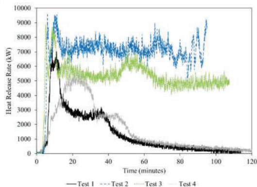
Figure 7: Heat release rate curves from WOODWISE Tests #1 through #4.
