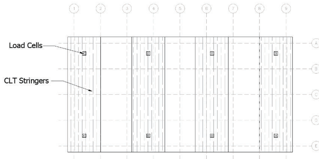
Figure 3: Locations of load cells and CLT stringers.
