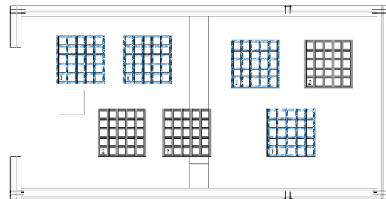
Figure 6: Schematic of wood cribs layout for Test #4. Locations with a blue crib and "1" indicate only one crib placed there. Locations with a gray crib and "2" indicate two cribs were stacked in that location.
