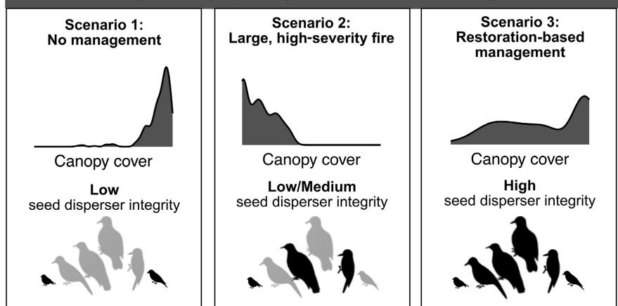
Figure 3. A worked example of monitoring animal communities for ecological integrity using bird community data from Colorado. (1) The combination of expanding data sources and statistical approaches leads to (2) an improved understanding of the functional composition of seed-dispersing birds across a range of habitat conditions, which in turn can lead to (3) predictions of the integrity of seed-dispersing bird communities given a range of land management decisions. Figure was created by Ana Miller-ter Kuile and Jamie S Sanderlin. Bar graph icon is from streamlinehq.com (CC-0 license). Vector images of birds and trees were created by Jamie S Sanderlin. In (2), horizontal lines within boxes depict median values, boxes represent the interquartile range (25th–75th percentiles), whiskers (vertical lines) represent 1.5×interquartile range, and solid circles depict outliers.
