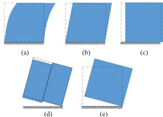
Figure 1: Deformation modes considered (a) Bending, (b) Shear, (c) Longitudinal shear fastener slip (d) Transverse shear fastener slip, and (e) Anchorage slip.
