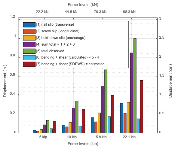
Figure 7: Contribution of fastener deformation to total diaphragm deformation for positive cycle, ASD = 70.3 kN (15.8 kip), LRFD = 98.3 kN (22.1 kip)
