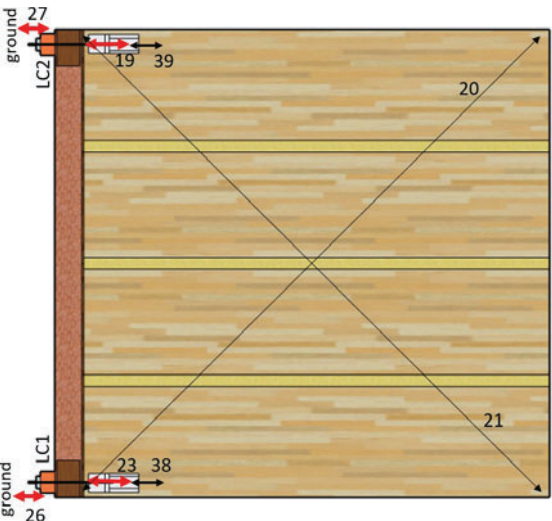
Figure 4: String pot and hold-down layout on the top of the diaphragm
