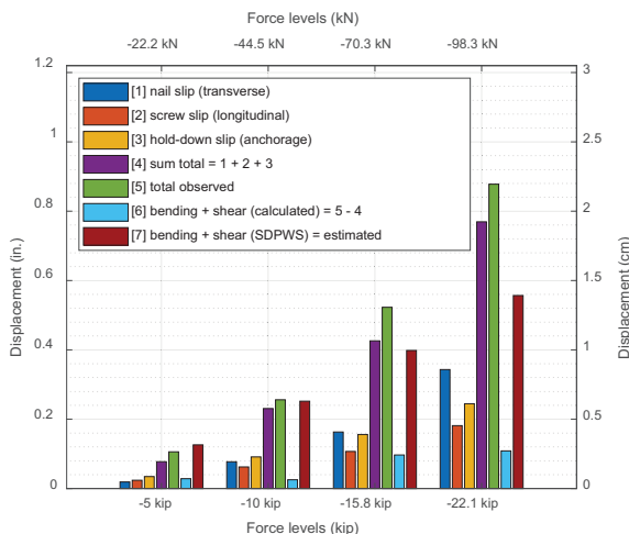
Figure 8: Contribution of fastener deformation to total diaphragm deformation for negative cycle, ASD = 70.3 kN (15.8 kip), LRFD = 98.3 kN (22.1 kip)
