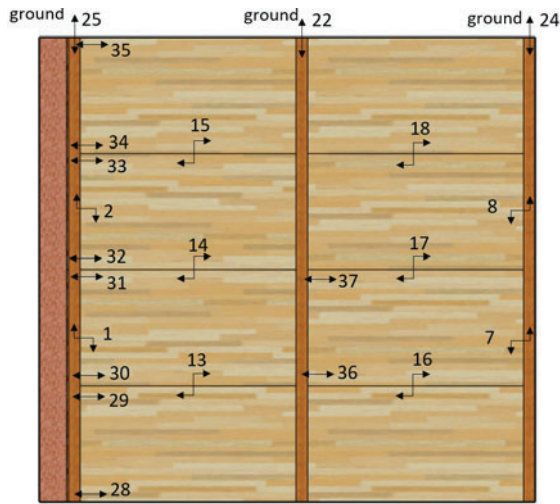
Figure 5: String pot layout on the bottom of the diaphragm
