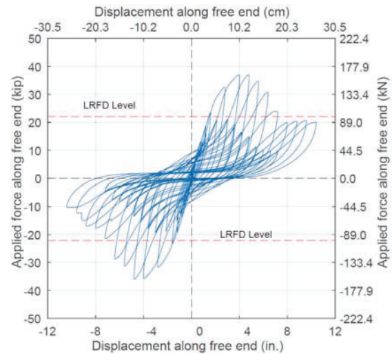
Figure 6: Force vs displacement hysteresis for the diaphragm test
