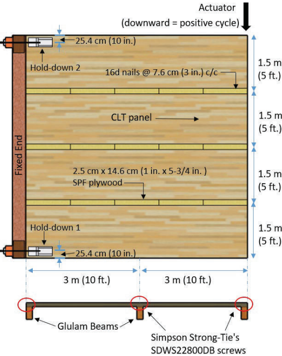
Figure 2: Layout for the diaphragm test
