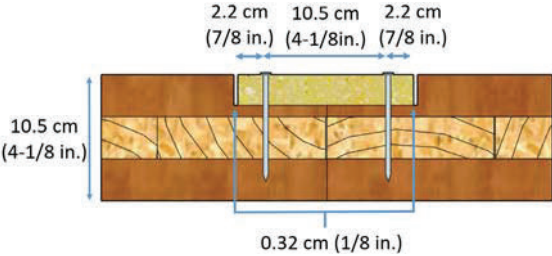
Figure 3: Surface spline detail
