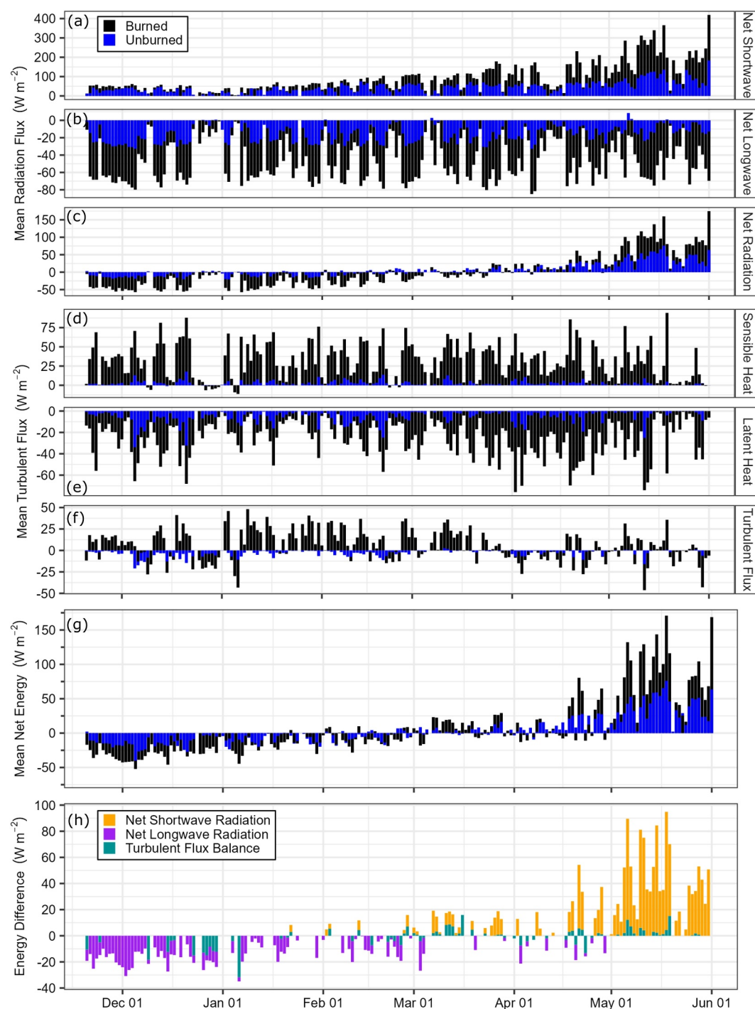
Figure 5. (a) Mean daily net shortwave, (b) longwave, and (c) radiation flux for the burned and unburned automated weather station (AWS) sites. Mean daily (d) sensible, (e) latent, and (f) total turbulent heat fluxes for the burned and unburned AWS sites. (g) Mean daily net energy at the burned and unburned AWS sites. (h) Daily difference between the mean daily net energy at the burned and unburned sites (burned minus unburned), and the proportion of the net difference attributed to each energy balance component.
