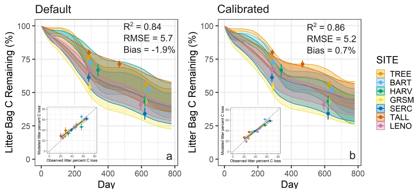
FIGURE 2 | Litter mass remaining in (a) default and (b) calibrated models compared to observations. Shading shows minimum and maximum decomposition predictions from the model, including variability due to three litter types and three soil moistures, and for the calibrated model, three parameter sets ( n=9 and n=27 simulations per site for default and calibrated results, respectively). Points with 95% confidence intervals show variability in observed litterbag mass loss at collection time points 1 and 2. Insets show comparison of modeled and observed decomposition, with dashed line depicting the 1:1 line. Sites are ordered from coldest (TREE) to warmest (LENO).
