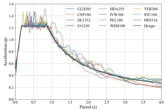
Figure 6. Eight-story building TBRB braced frame matched earthquake spectra for 10.0% probability of exceedance in 50 years.
