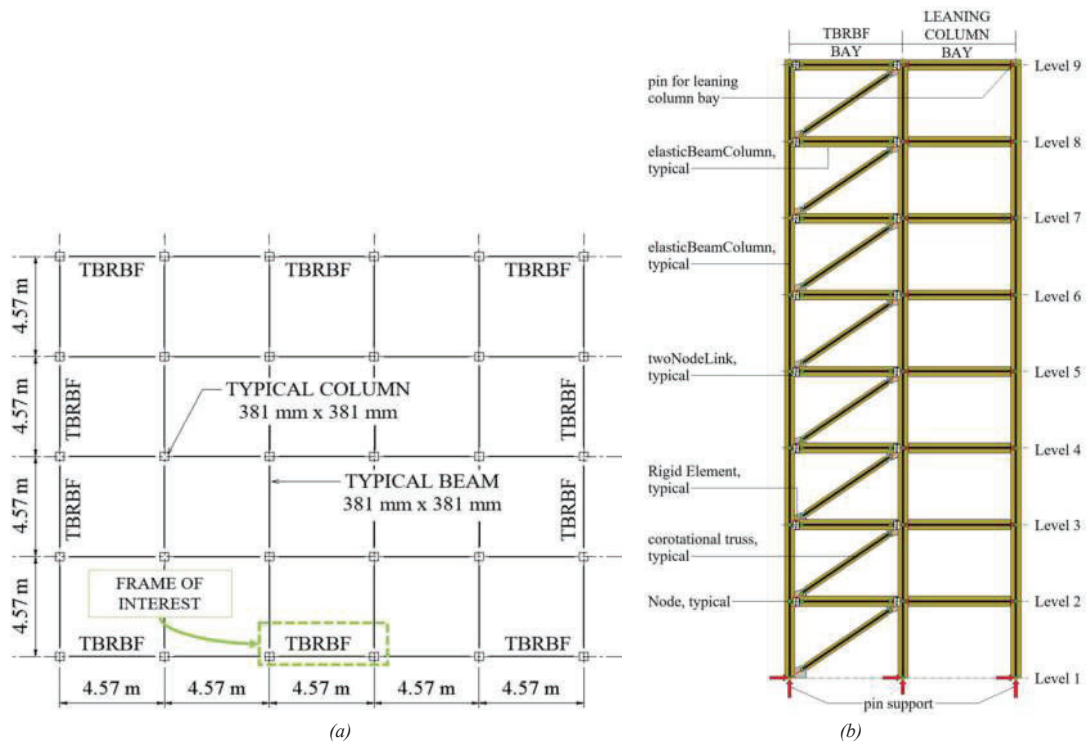
Figure 5. Eight-story building: (a) plan view of theoretical TBRB braced frame office building; (b) eight-story building TBRB braced frame model.
