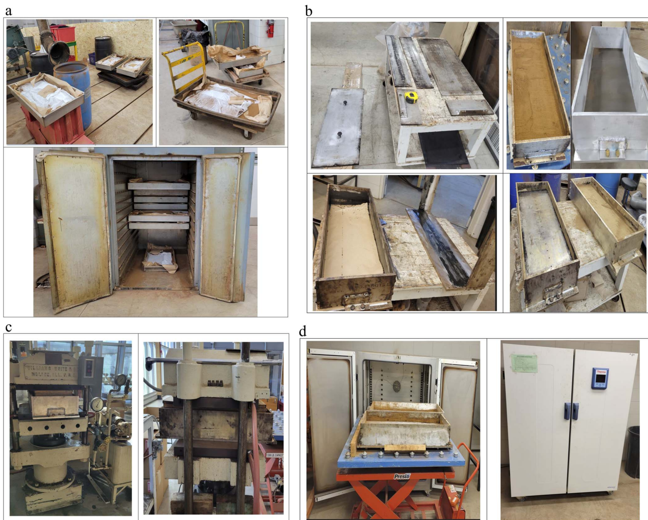
Figure 1.—(a) Drying lignin, (b) preparation and filling the lignin-foam molding frame, (c) pressing the molding frame, and (d) transferring lignin-foam blocks to the 240°C oven.
