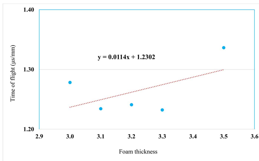
Figure 4.—Regression among lignin-foam block thickness. P = 0.9195 ; R^2 = 0.1743 .
