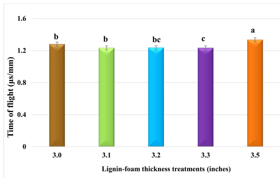
Figure 5.—Main effect of 3.0- to 3.5-in. thickness on the acoustic velocity of lignin foam blocks. Treatment means within the same column within effect without common lowercase letters are significantly different. Number of replications per treatment combination is 12 or 9; P < 0.001 ; SEM = 0.0246.
