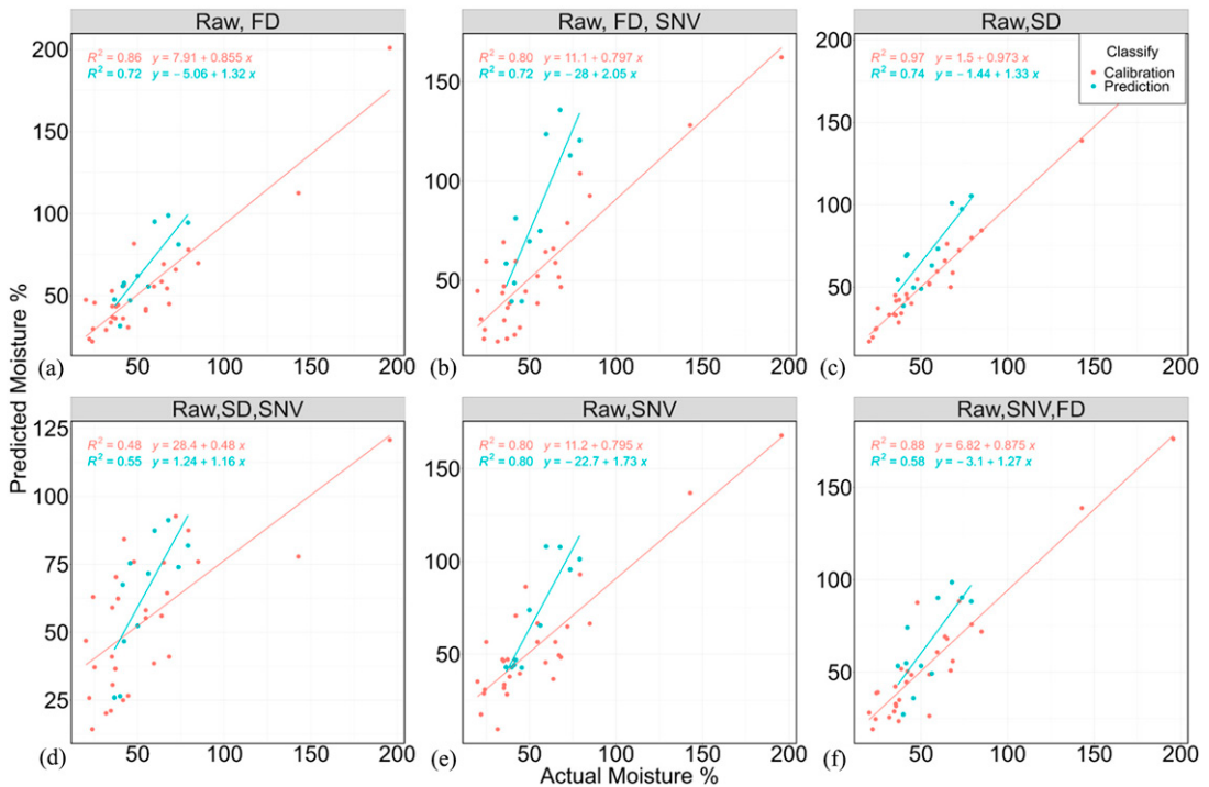
Figure 3. Predicted vs actual wood MC by partial least square regression models fitted with spectra subjected to different pre-processing treatments. (a-f) Effects of different spectral preprocessing method combinations on wood moisture prediction. FD, first-order derivative; SD, second-order derivative; SNV, standard normal variate.
