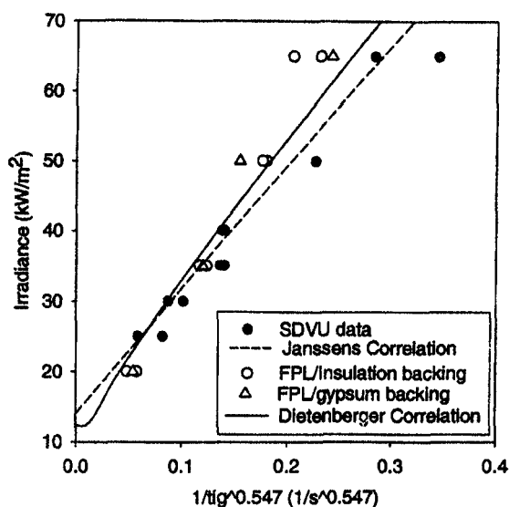
Figure 3. Correlation to piloted ignition data of Douglas-fir plywood (ASTM) (ISO 5)
