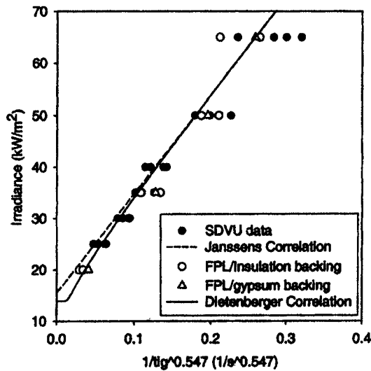
Figure 7. Correlation to piloted ignition data of Southern pine plywood (ISO 10)
