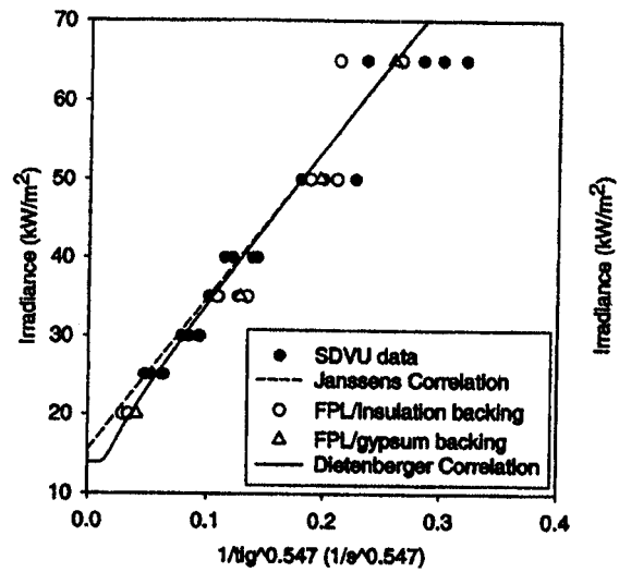
Figure 6. Correlation to piloted ignition data of Gypsum X (ISO 1)
