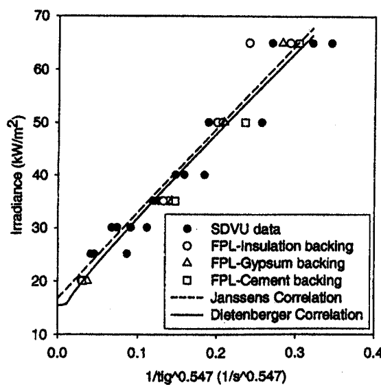
Figure 2. Correlation to piloted ignition data of redwood (ISO 14)
