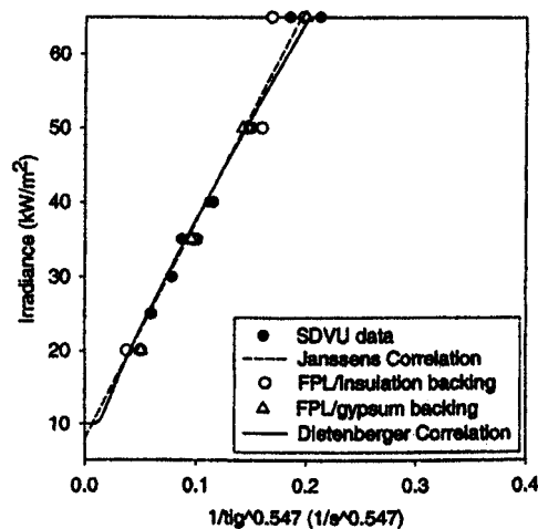
Figure 9. Correlation to piloted ignition data of Particleboard (ISO 11)
