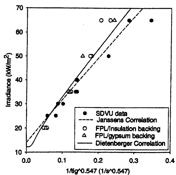
Figure 2. Correlation to piloted ignition data of oriented strand board (OSB) (ISO 12)
