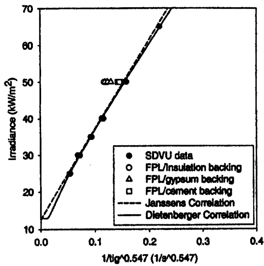
Figure 5. Correlation to piloted ignition data of Gypsum X (ISO 1)
