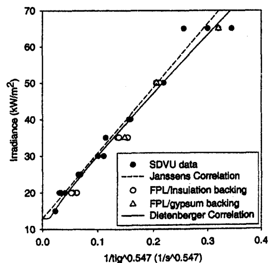
Figure 4. Correlation to piloted ignition data of Douglas-fir plywood (ASTM) (ISO 5)
