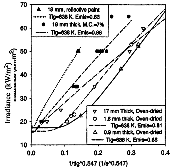
Figure 1. Prediction of redwood piloted ignition with varying irradiance, thickness, moisture content, and surface emissivity using Diitenberger's correlation
