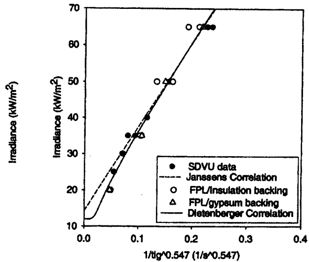
Figure 8. Correlation to piloted ignition data of Hardboard (ISO 13)
