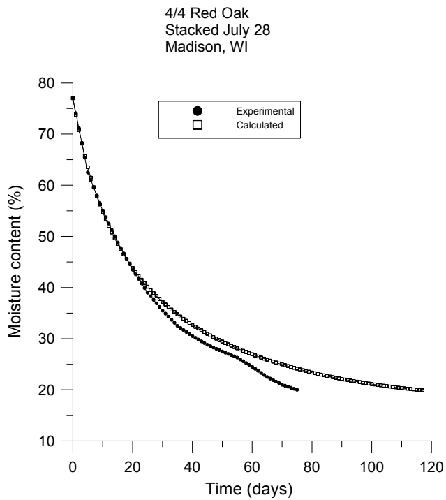
Figure 1—Moisture content time graphs for air drying 1-in.-thick red oak in Madison, Wisconsin, with stacking started in (a) January, (b) May, (c) July, and (d) October.
