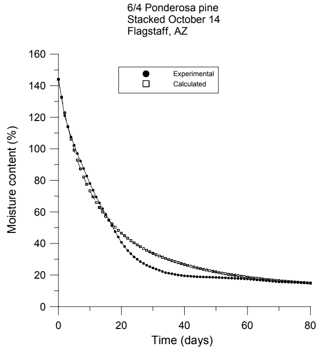
Figure 4—Moisture content time graphs for air drying 1.5-in.-thick ponderosa pine in Flagstaff, Arizona, with stacking started in (a) January, (b) May, (c) July, and (d) October.
