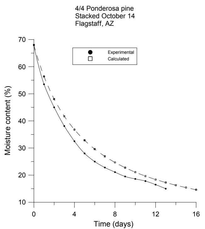
Figure 3—Moisture content time graphs for air drying 1-in.-thick ponderosa pine in Flagstaff, Arizona, with stacking started in (a) January, (b) May, (c) July, and (d) October.
