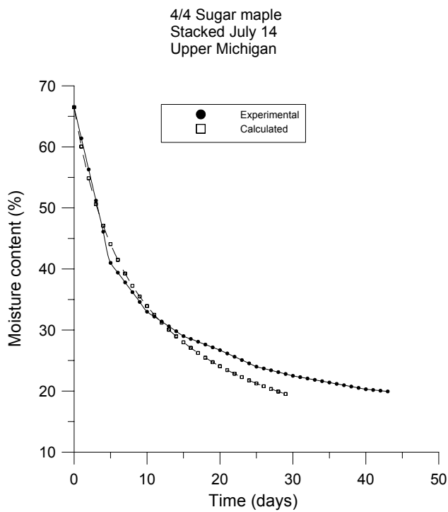
Figure 2—Moisture content time graphs for air drying 1-in.-thick sugar maple in upper Michigan, with stacking started in (a) January, (b) May, (c) July, and (d) October.
