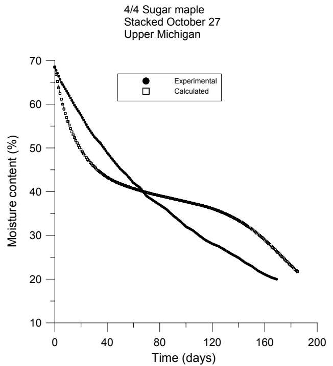
Figure 2—Moisture content time graphs for air drying 1-in.-thick sugar maple in upper Michigan, with stacking started in (a) January, (b) May, (c) July, and (d) October.
