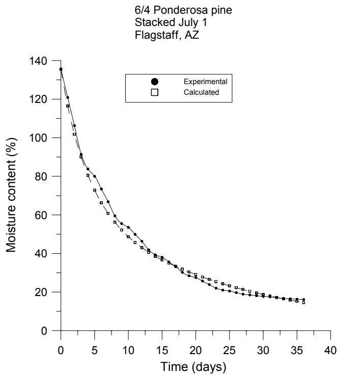
Figure 4—Moisture content time graphs for air drying 1.5-in.-thick ponderosa pine in Flagstaff, Arizona, with stacking started in (a) January, (b) May, (c) July, and (d) October.
