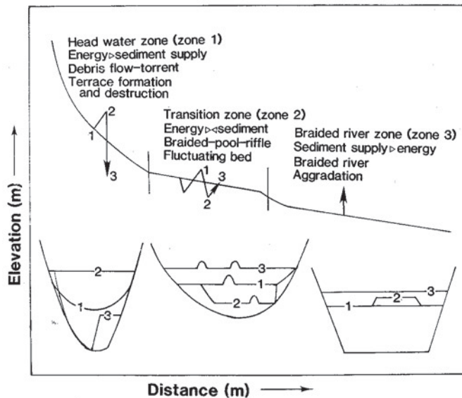
Figure 9—Idealized longitudinal profile divided into headwater, transitional, and braided zones. Arrows denote mean behavior of bed through a sedimentation cycle. Cross sections correspond to each zone over time, progressing from 1 to 3.
