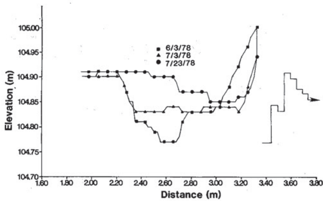
Figure 6—Cross section 5, zone 2, basin 1200. Schematic diagram at the right illustrates channel-bed behavior during the study period.
