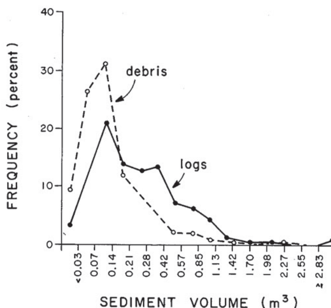
Figure 3—Frequency of occurrence of sediment volume by size classes stored behind debris and log obstructions.
