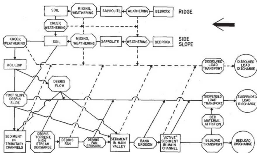
Figure 2—Sediment-budget model for the Rock Creek basin, central coastal Oregon: rectangles, storage sites; octagons, transfer processes; circles, outputs; solid lines, transfer of sediment; and dotted lines, migration of solutes (from Dietrich and Dunne 1978).
