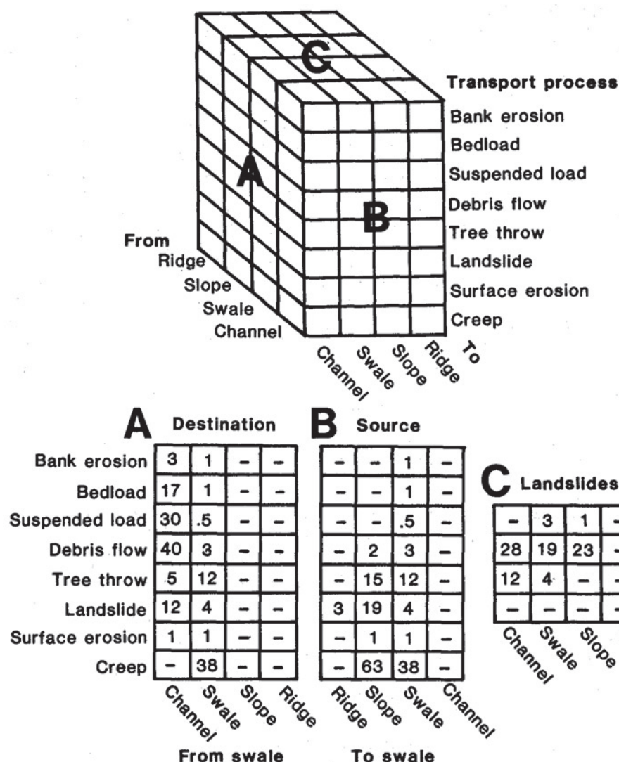
Figure 1—Hypothetical three dimensional matrix for tabulation of material transfer rates between storage locations in a forested basin. Material is moved from source A to location B by transport process C. Hypothetical tabulations, in t/km 2 per year, are shown in 1A, 1B, and 1C. Change in storage at a location can be calculated by subtracting total output from total input at that location. In the example given, the rate of change of the volume of material stored in swales would be (total (1B) - total (1A)) = -5 t/km 2 per year.
