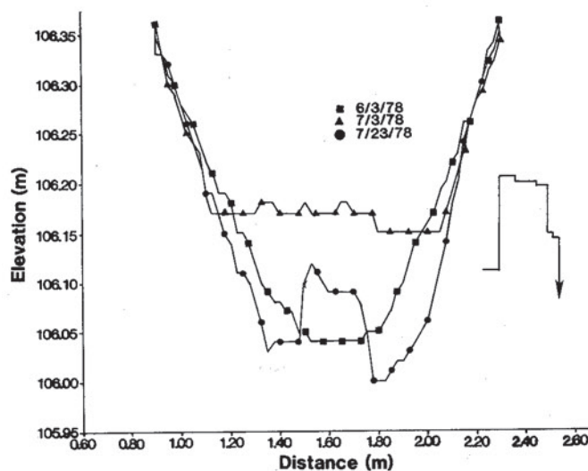
Figure 7—Cross section 7, lower zone 1, basin 1200. Schematic at the right illustrates the behavior of the channel bed over the period of record.
