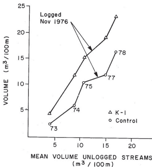
Figure 6—Double mass analysis showing volume of sediment storage behind obstructions before and after logging.
