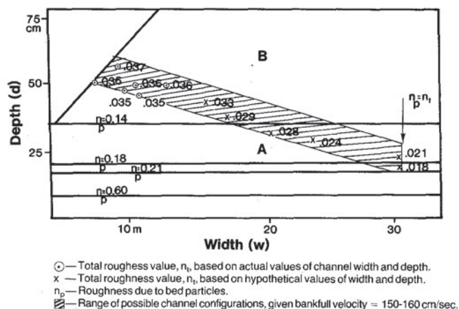
Figure 6—Velocity and roughness constraints on the Big Beef Creek channel configuration at bankfull discharge (relationships determined from equations 3, 4, and 6).
