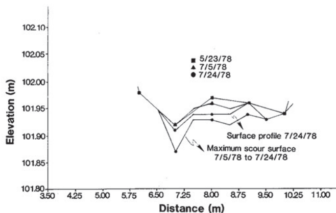
Figure 8—Cross section 1, lower zone 3, drainage basin 1200. Lower profile for 7.24.78 is the surface of greatest scour during the survey interval. Upper profile for 7.24.78 is existing surface at time of survey.
