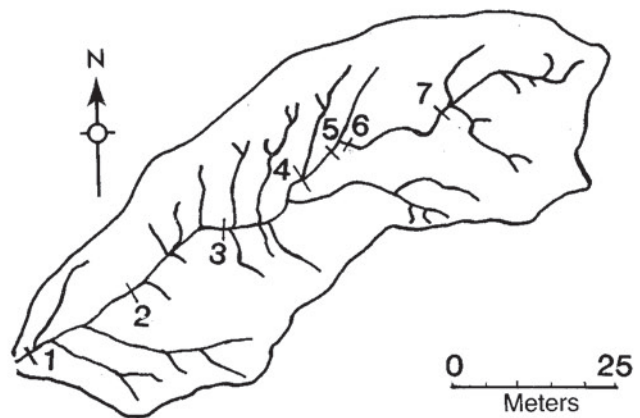
Figure 3—Basin 1200 showing drainage divide, drainage pattern, and cross-section locations.
