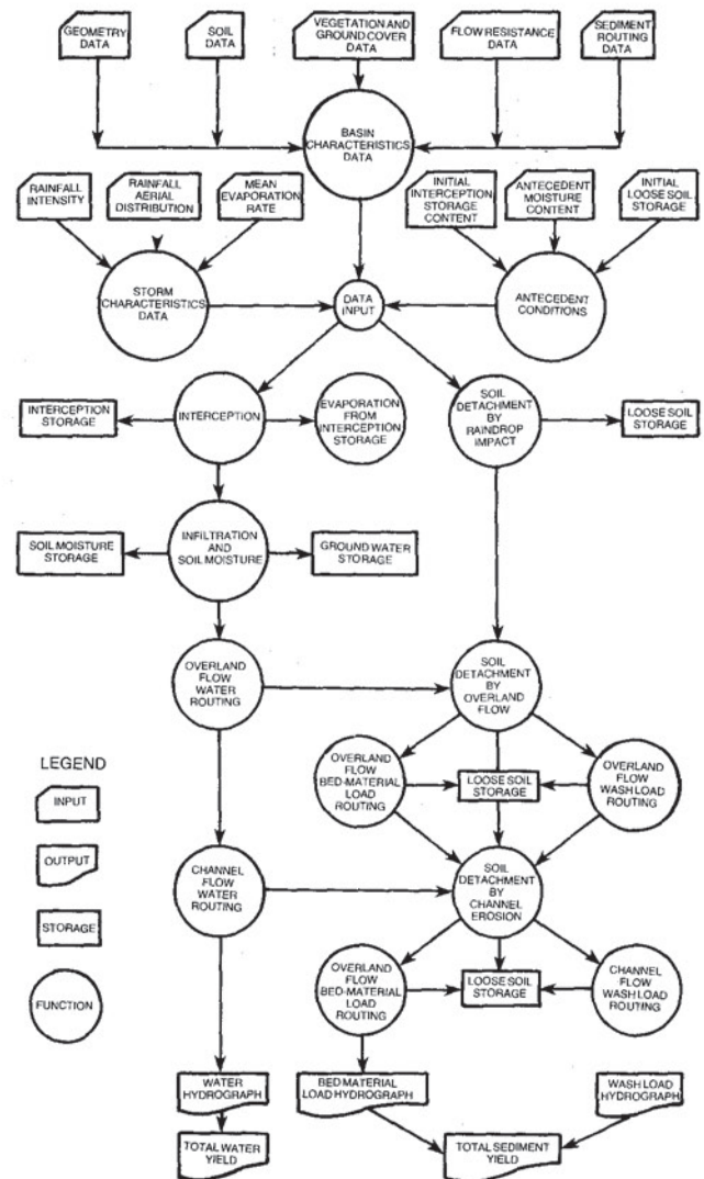
Figure 2—Flow chart for the drainage-basin sediment and routing model.
