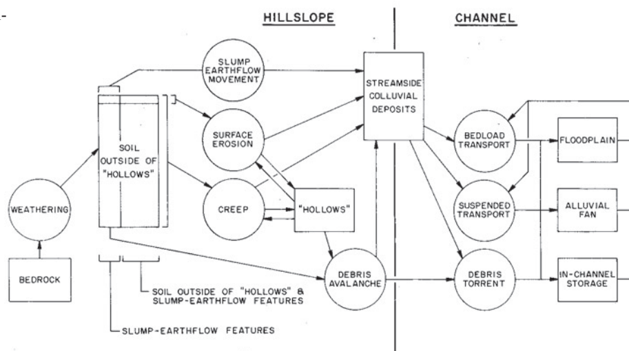
Figure 1—Simplified flow chart of relationships among storage sites (boxes) and transport processes in steep, volcanic terrane in the western Cascades, Oregon.
