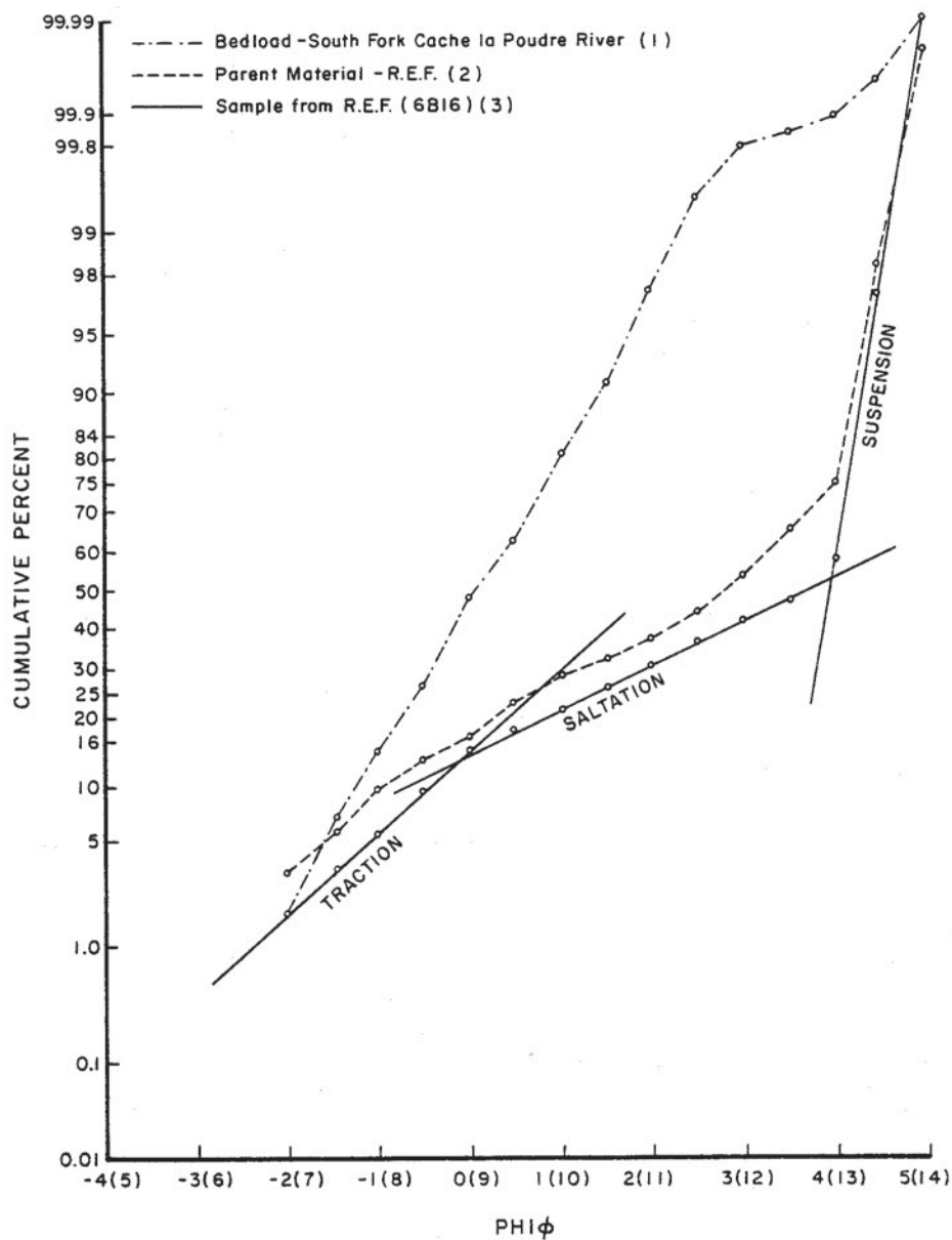
Figure 2—Log probability plots of: (1) bedload sample from the South Fork of the Cache la Poudre River, material" used in R.E.F.; (3) sample 6B16 from the R.E.F.
