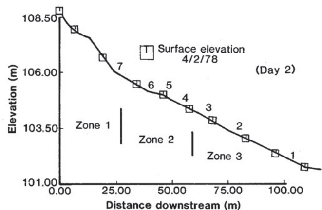
Figure 4—Longitudinal profile of channel in basin 1200. Numbers refer to cross-section locations.
