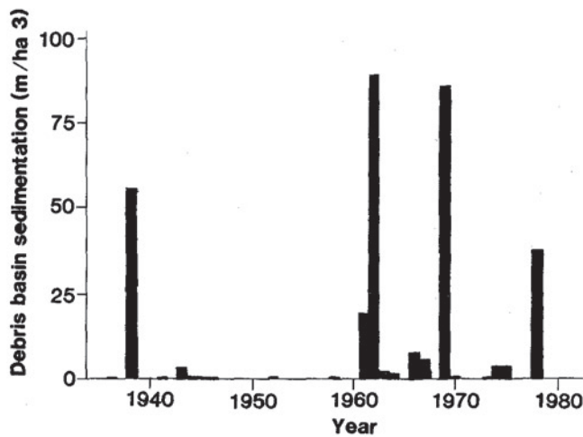
Figure 3—Annual accumulate in Bell IV debris basin. (Hydrologic Year 1961 and 1962 record combined, sediment distributed between them based on records from nearby basins. Hydrologic Year 1978 is ocular estimate, survey data not yet available.)
