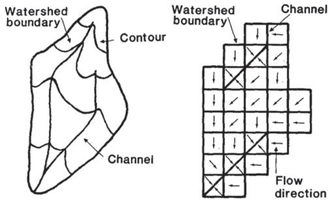
Figure 1—Example of drainage-basin segmentation.
