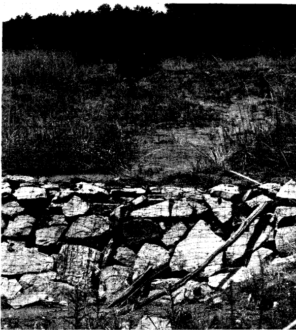
(Left) Check dams of loose rock, reinforced by woven wire were used to control erosion. Manitou Experimental Forest, Colorado.
