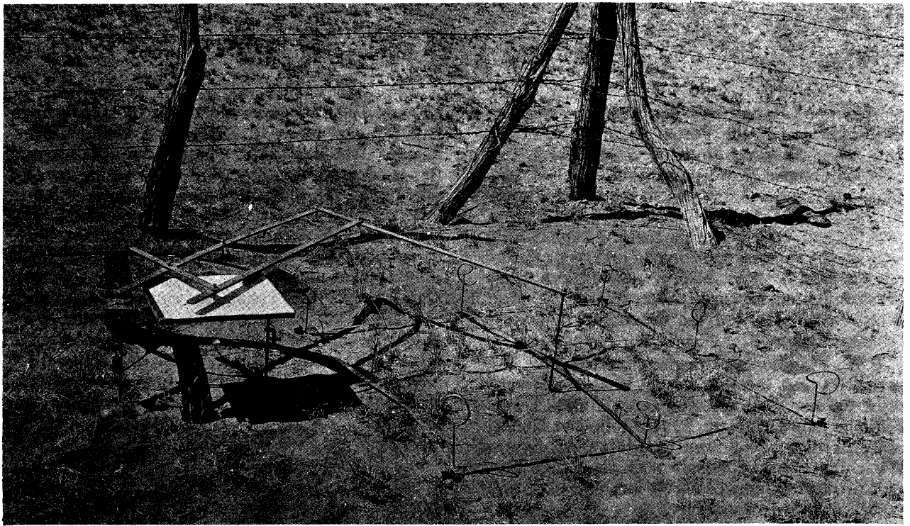
R. R. Hill's pantograph, set up for measuring black grama quadrat. Jornada Experimental Range, New Mexico, 1924.
