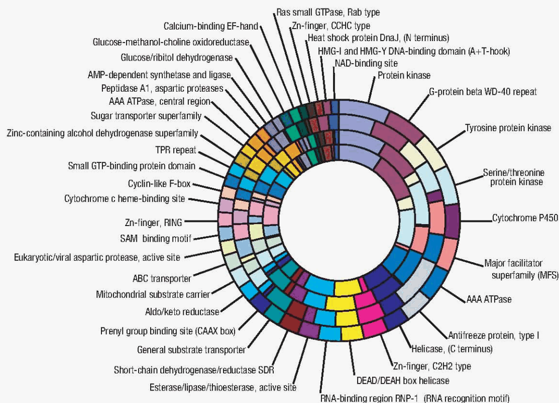
Figure 2 Schematic showing the InterPro version 5.3 (ref. 12) domains in P. chrysosporium (outer ring), N. crassa , S. pombe and S. cerevisiae (inner ring). InterPro contains the combined protein signature databases of Swiss-prot, TrEMBL, PROSITE, PRINTS, Pfam, ProDom, SMART and TIGRFAM. Note the large difference between the three organisms in the size of bands corresponding to the cytochrome P450 domain (IPR001128) indicating the expansion of this gene family in P. chrysosporium . Type I Antifreeze domains (IPR000104) are artifacts attributed to a common tripeptide repeat, Ala-Ala-Thr. The number of sequences per domain is listed separately (Supplementary Table 3 online).
