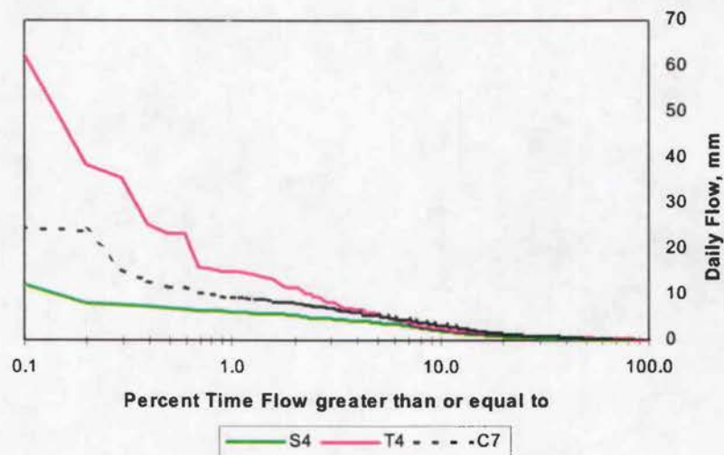
Figure 4. Measured daily flow duration data for three watersheds (S4, T4 and C7) for 1998-2001.
