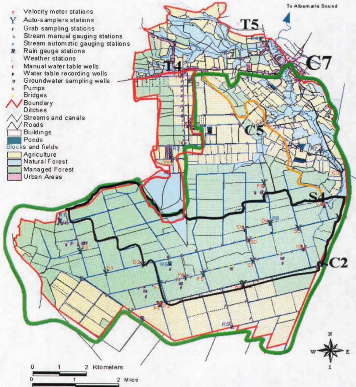
Figure 1. A map of the 10,000 ha lower coastal plain study site showing watersheds S4, T4, and C7 boundaries along with drainage network and monitoring stations.
