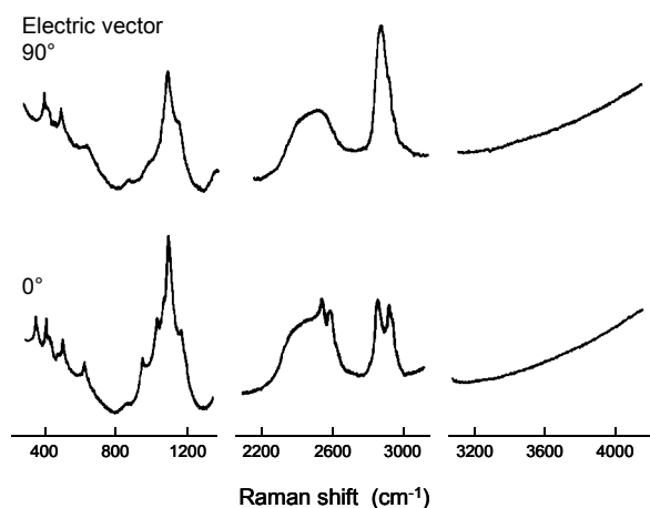
Fig. 5. Raman spectra of mercerized ramie fiber in D 2 O, measured by laser beam with electric vector at 90 and 0° to the fiber axis. This ramie fiber was treated with 30 % NaOD/D 2 O, and then washed with D 2 O (never-dried).
