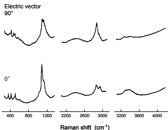
Fig. 3. Raman spectra of ramie fiber in D 2 O, measured by laser beam with electric vector at 90 and 0° to the fiber axis.
