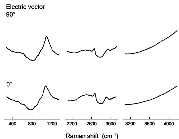
Fig. 4. Raman spectra of ramie fiber in 30 % NaOD/D 2 O, measured by laser beam with electric vector at 90 and 0° to the fiber axis.
