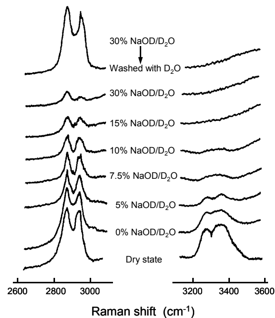
Fig. 2. Raman spectra (C-H and O-H stretching regions) of single ramie fiber subjected to various treatments. These spectra were measured by laser beam with electric vector parallel to the fiber axis.
