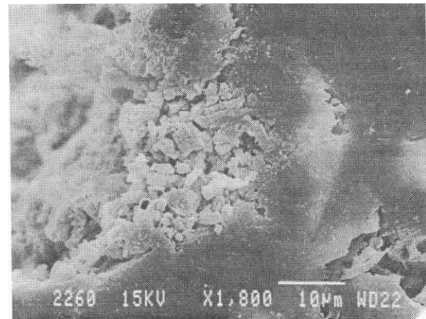
Figure 11. ~ SEM micrograph of UV degradation of a cross section of blend 3 taken at the surface of the specimen (1,800x).
