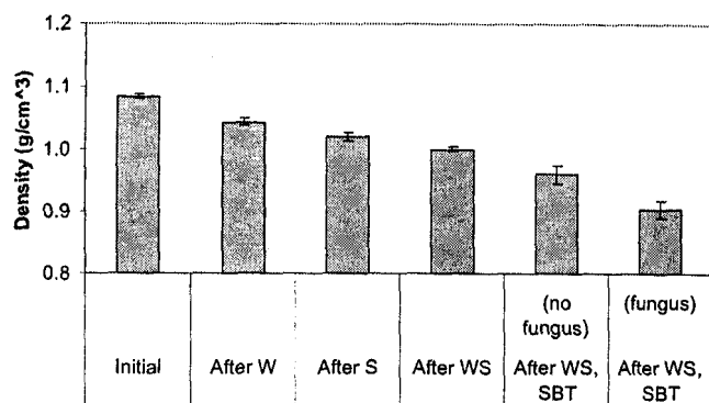
Figure 7. ~ Density reduction after various exposures with blend 1. SBT = soil block test.
