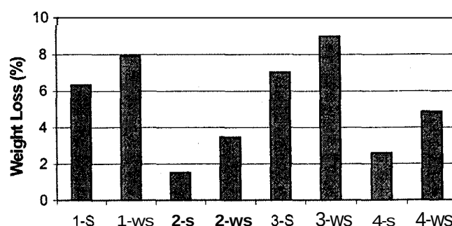
Figure 3. — The average weight loss after a 12-week modified soil block test. (No fungus correction.)
