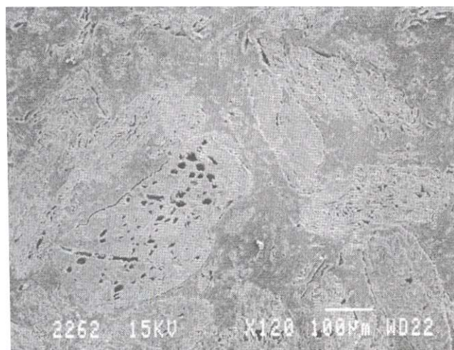
Figure 8. ~ SEM micrograph of the core of a cross section of blend 3 (UV package) with no preconditioning or decay (120x).
