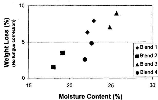
Figure 6. ~ The correlation between weight loss and moisture content after exposure to G. trabeum in the modified soil block test for 12 weeks.
