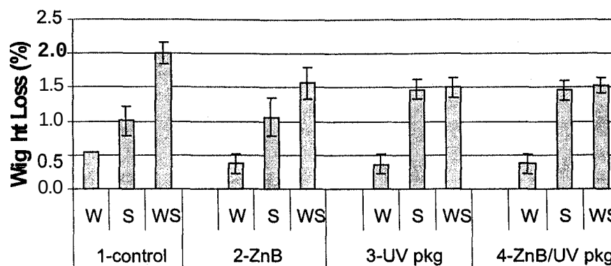
Figure 1. — The average weight loss of specimens after preconditioning. W = weathering, S = watersoaking, and WS = weathering then water soaking.
