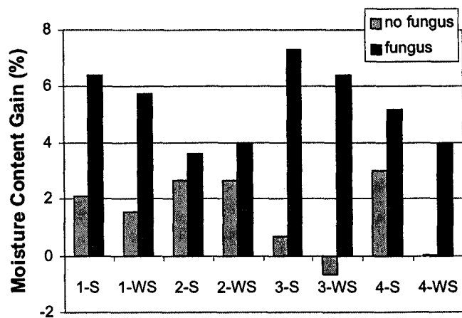
Figure 5. ~ The average moisture content gained during the 12-week soil block test.
