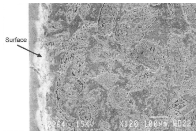
Figure 9. ~ SEM micrograph of the surface of a cross section of blend 3 WS after exposure to G. trabeum . (UV package, weathered, soaked, decayed, 120x.)
