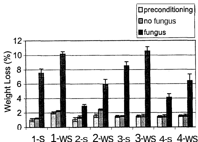
Figure 2. — The average weight loss after preconditioning or fungal decay testing.
