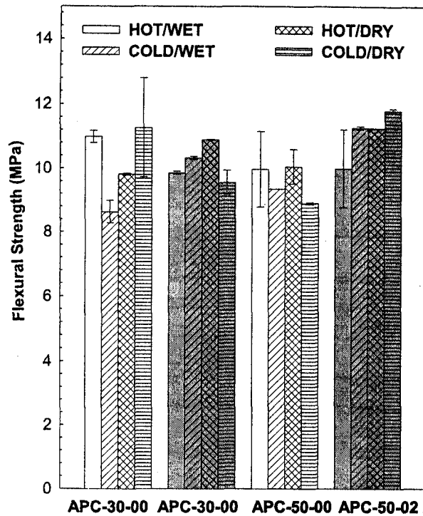
Figure 1. ~ Flexural strengths of APC-30s and APC-50s tested at room temperature after 7,000 hours conditioning.
