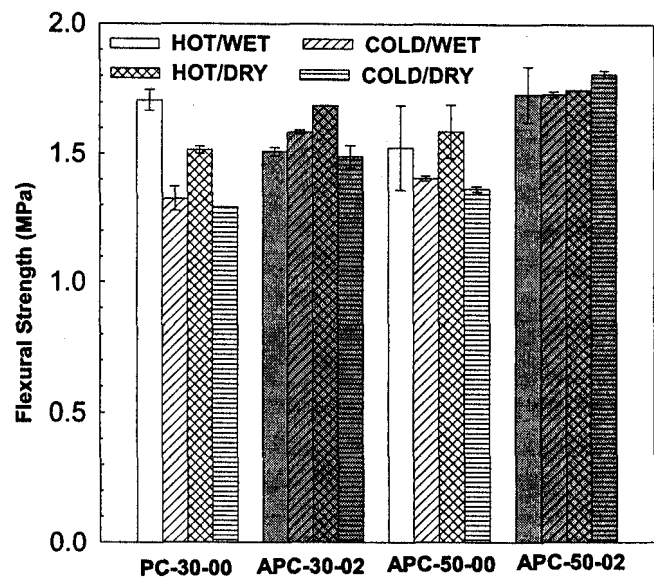
Figure 3. ~ Flexural strengths of APC-30s and APC-50s tested at elevated temperature (40°C) after 7,000 hours conditioning.
