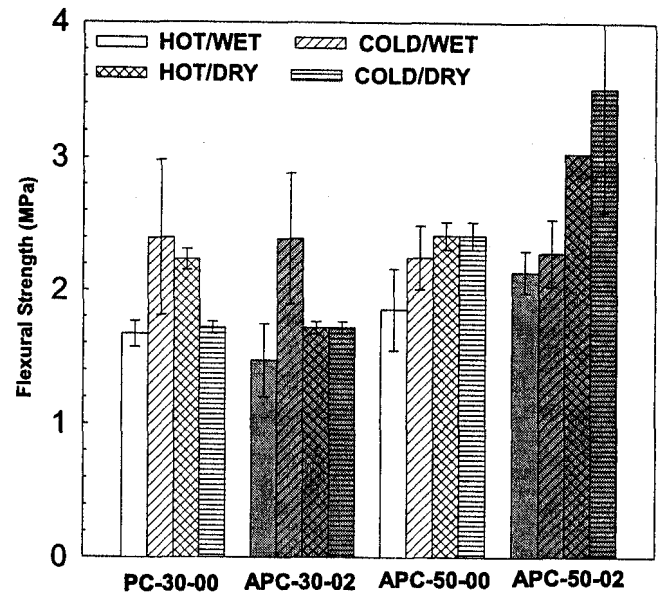
Figure 2. ~ Flexural strengths of APC-30s and APC-50s tested at near frozen temperature (4°C) after 7,000 hours conditioning.
