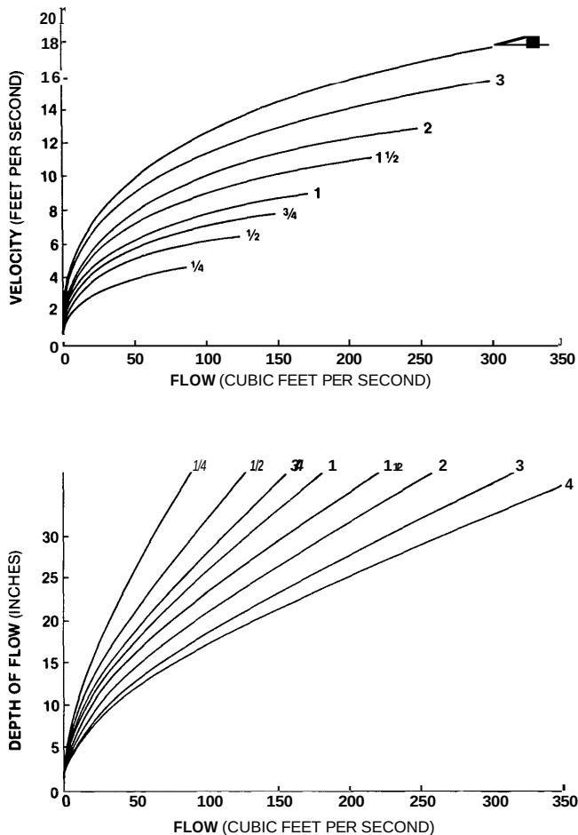
Figure 4--Velocity and depth-of-flow curves for a 7-foot by 5-foot 1-inch pipe-arch (after Evans and Johnston 1974).
