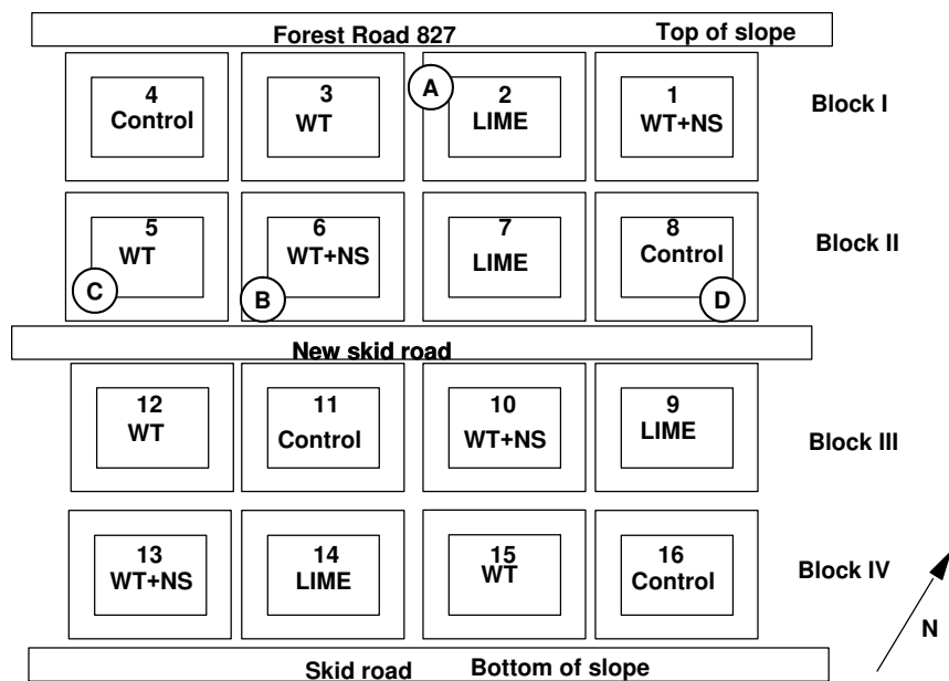
Figure 2.—Plot layout and treatment assignments, Fork Mountain Long-Term Soil Productivity Study. Letters within circles indicate location of characterization soil pits. See Appendix Table 19 for descriptions.
