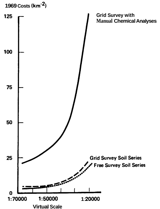
Figure 1.--The cost of soil survey in relation to virtual map scale (After Burrough and Beckett, 1971)
