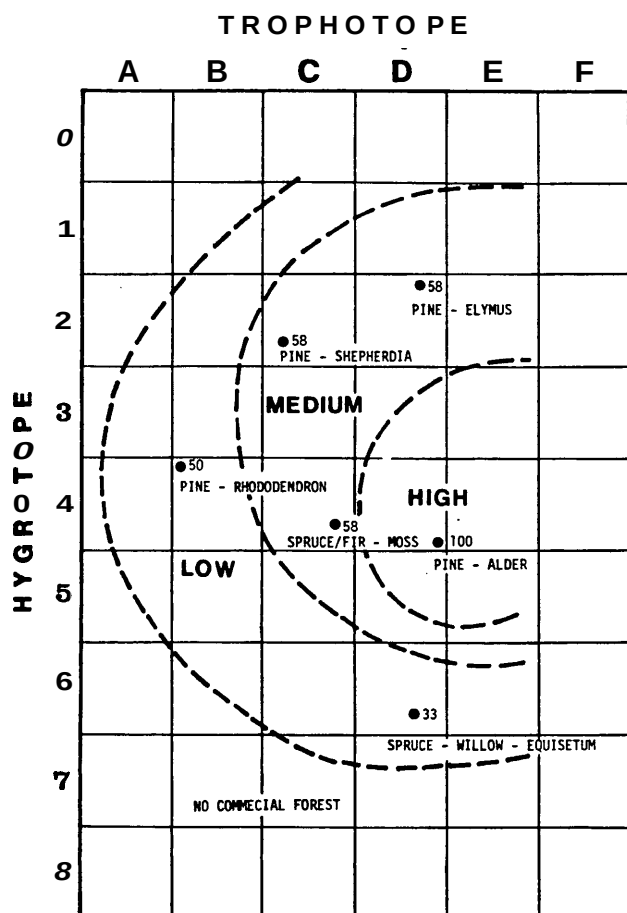
Figure 8.--Productivity potential map of the lower northern subalpine region of Alberta.
