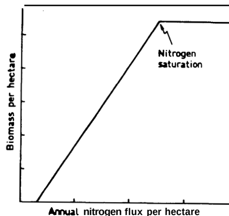
Figure 1.--Biomass production is linearly defined by the nitrogen flux in the ecosystem (after Ingestad et al. 1981).
