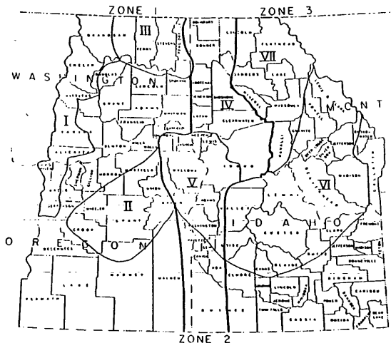
Figure 1.--The seven physiographic regions of the Intermountain Tree Nutrition Cooperative.
