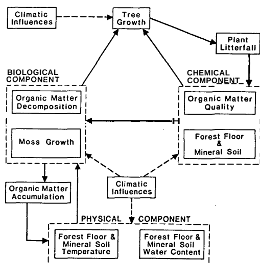
Figure 1. The relationship of factors controlling site quality to tree productivity.
