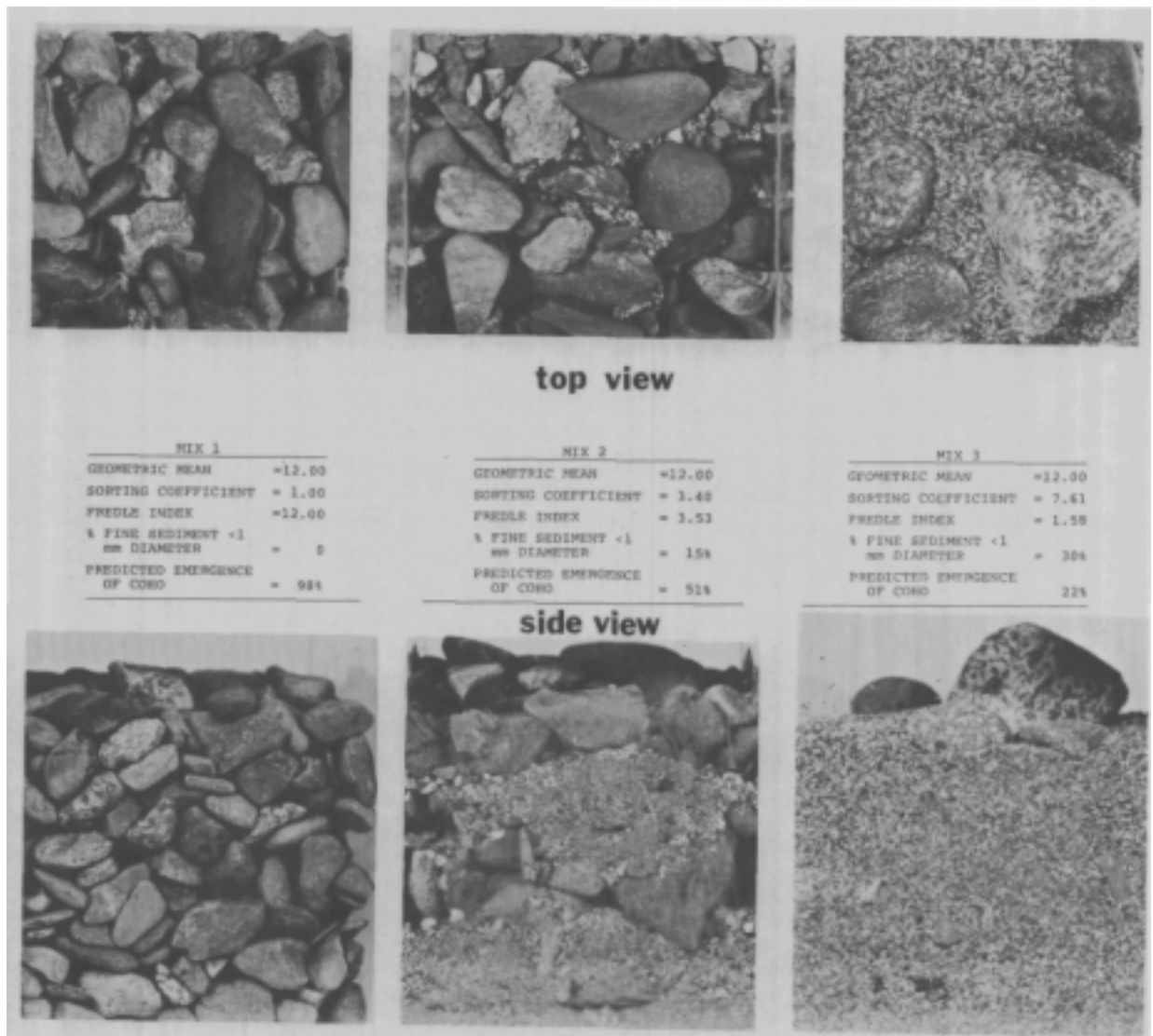
Figure 2.--Three gravel mixtures with a common geometric mean ( d_g ) but widely divergent distribution of particle sizes.
