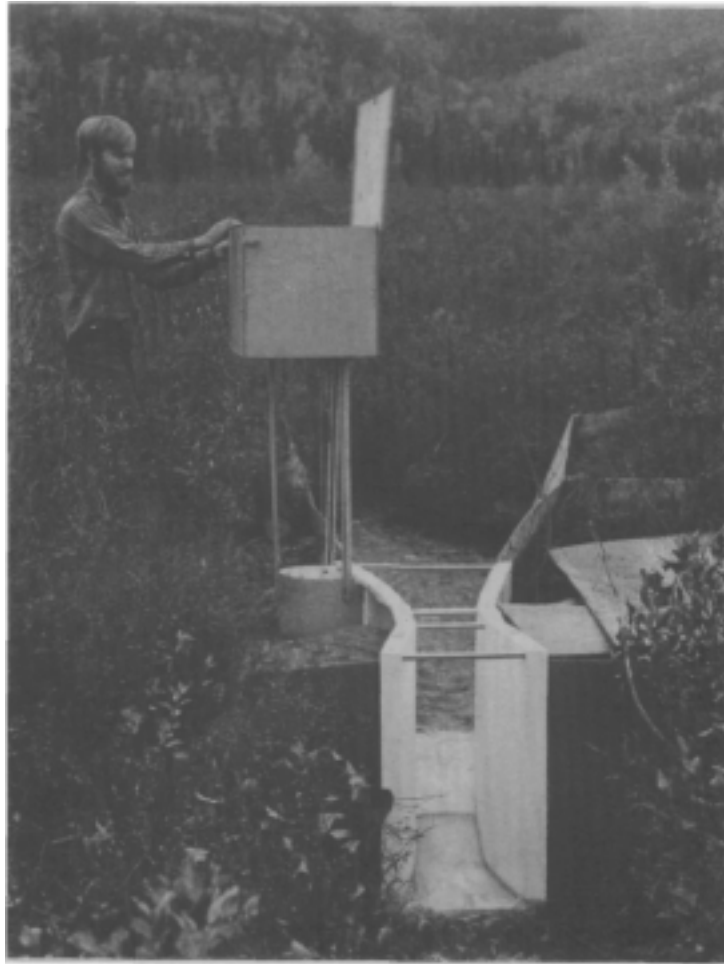
Figure 1.—Parshall flume in C-2 channel; view is upstream. Water-level recorder is in box above the stilling well.
