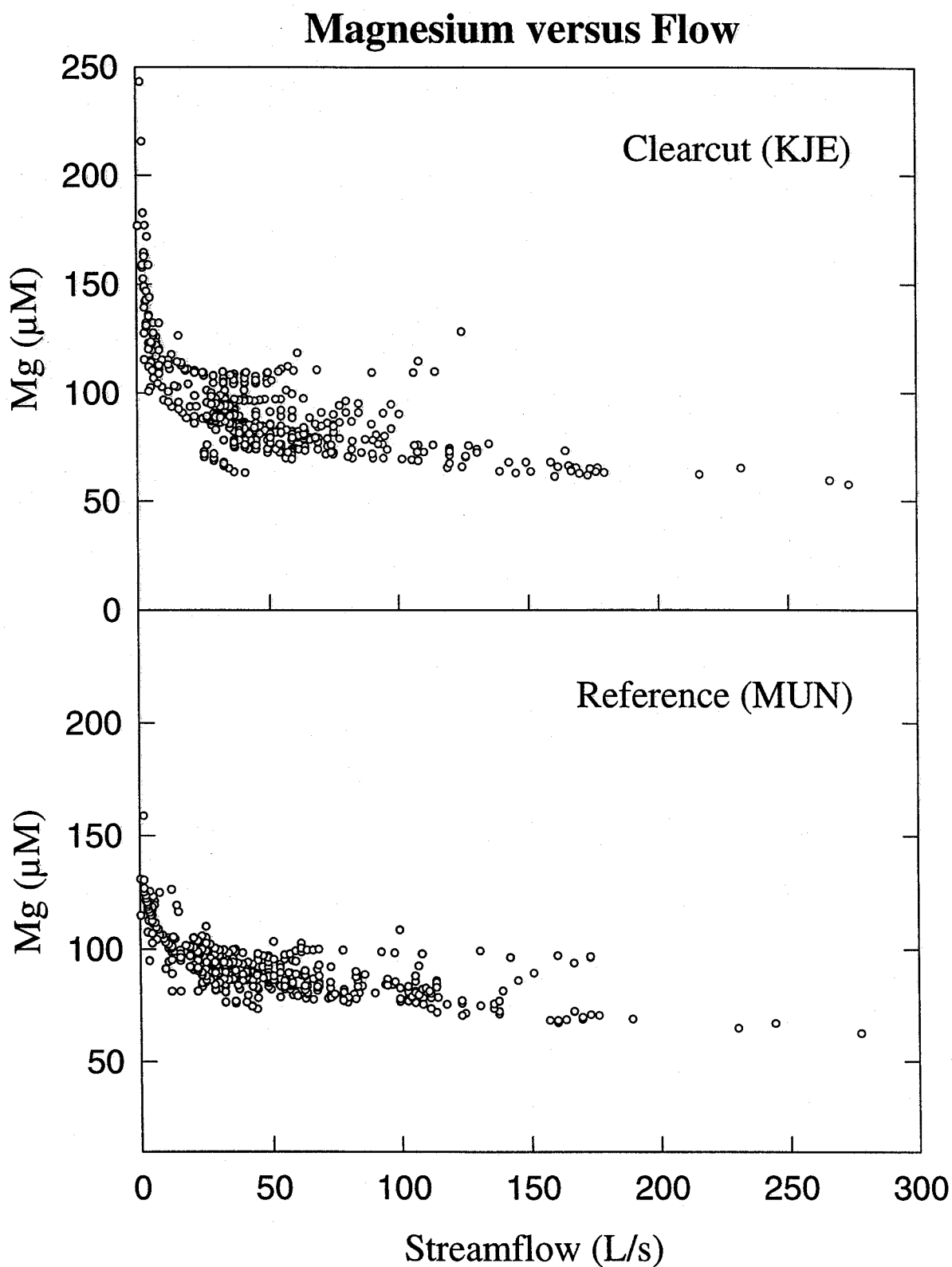
Fig. 26. Relationship between stream water magnesium concentrations and stream discharge for the reference (MUN) and clearcut (KJE) watersheds during the five year study period.
