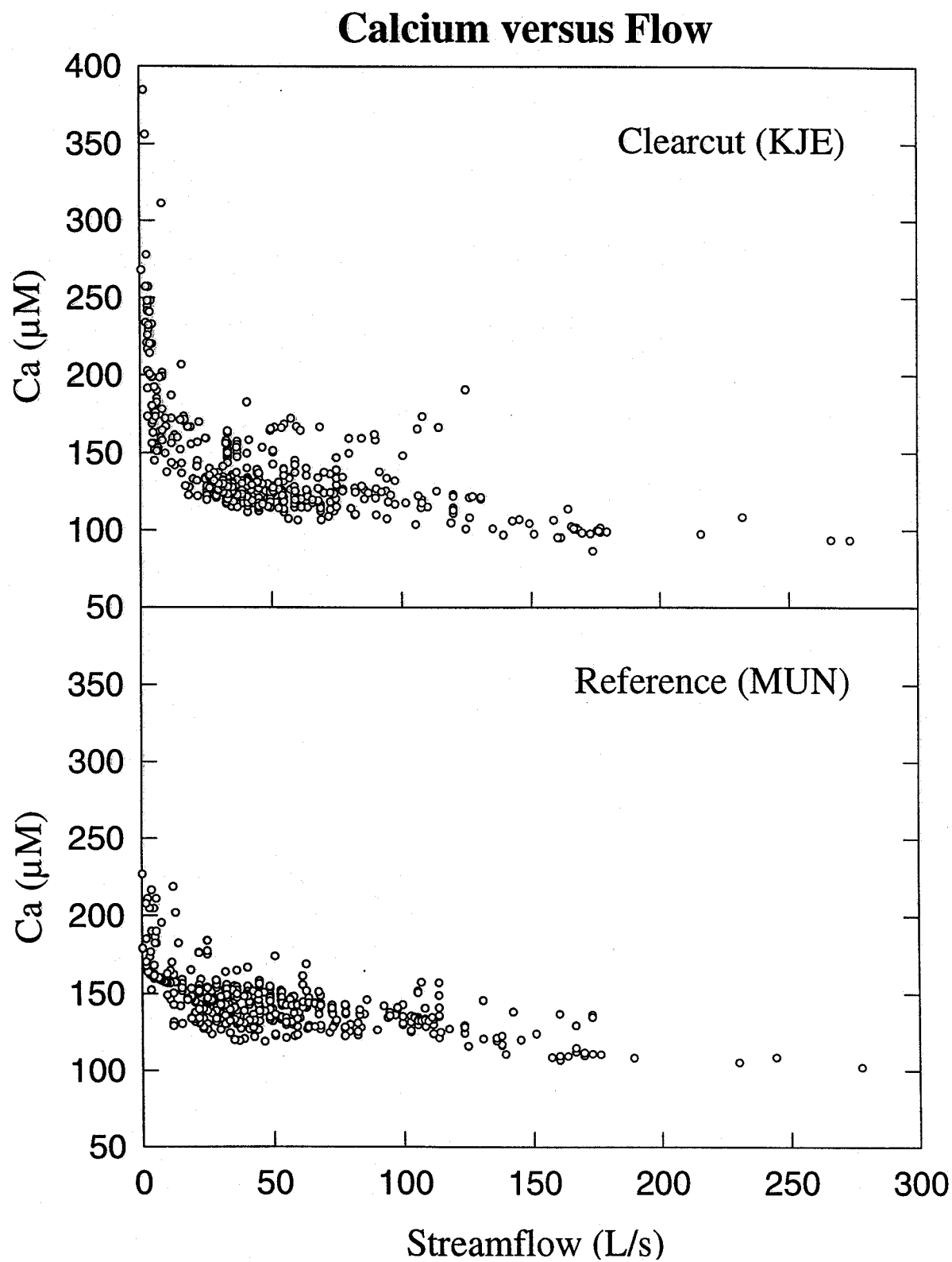
Fig. 25. Relationship between stream water calcium concentrations and stream discharge for the reference (MUN) and clearcut (KJE) watersheds during the five year study period.
