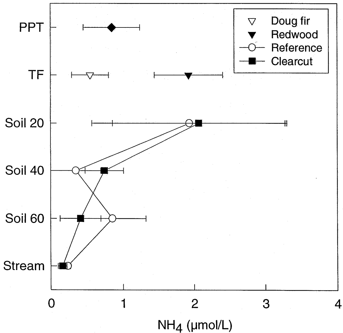
Fig. 13. Mean \pm standard deviation for ammonium in precipitation (PPT), canopy throughfall (TF), soil solutions at 20, 40 and 60 cm depths, and stream water for the period October, 1993 to June, 1996 in the clearcut (KJE) and reference (MUN) watersheds.
