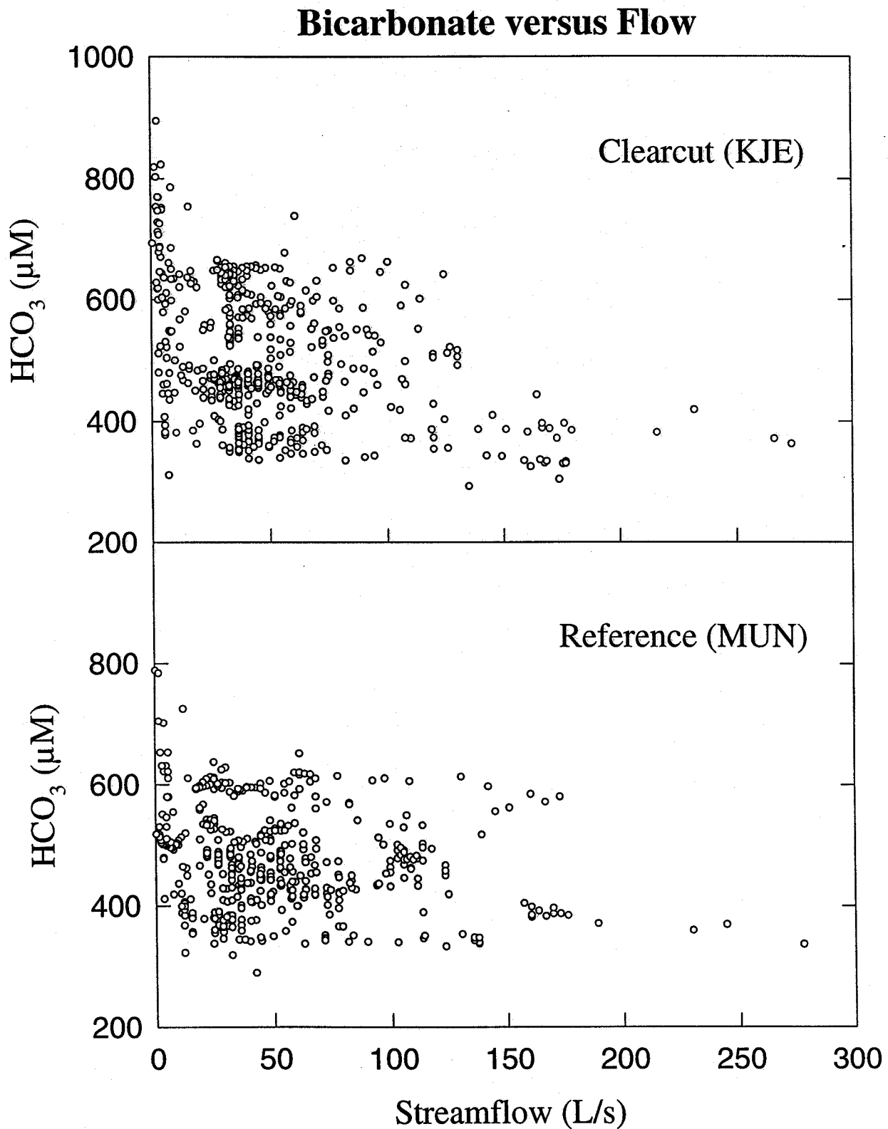
Fig. 32. Relationship between stream water bicarbonate concentrations and stream discharge for the reference (MUN) and clearcut (KJE) watersheds during the five year study period.
