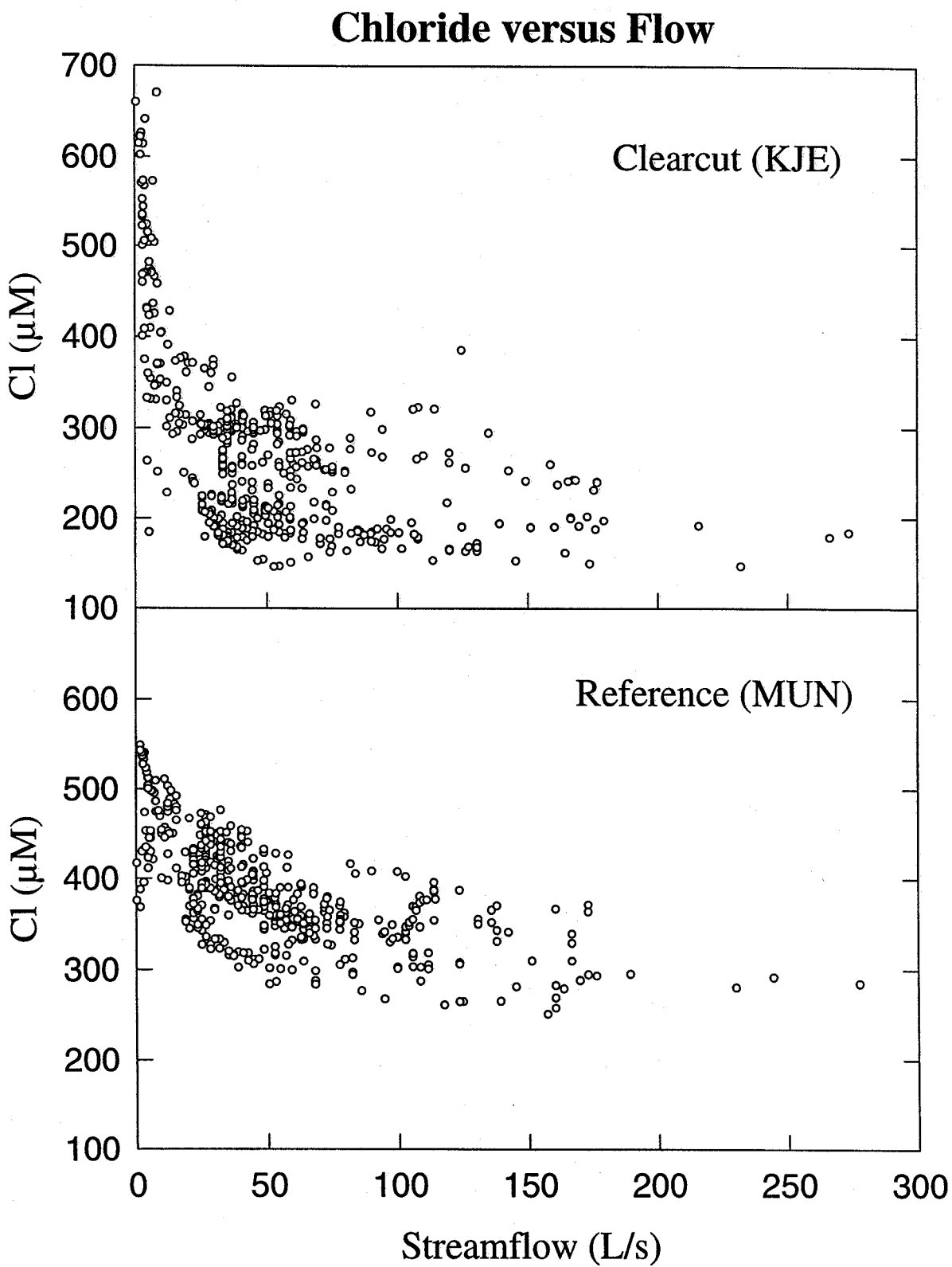
Fig. 29. Relationship between stream water chloride concentrations and stream discharge for the reference (MUN) and clearcut (KJE) watersheds during the five year study period.
