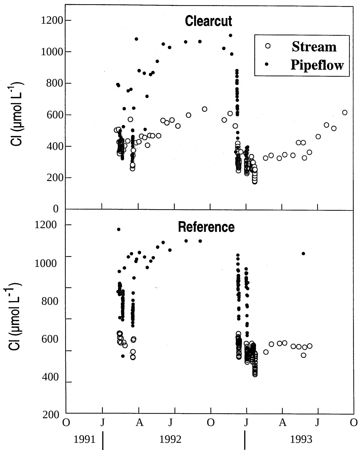
Fig. 38. Comparison of stream water and pipeflow chloride concentrations for the reference (MUN) and clearcut (KJE) watersheds during the 1991 - 1993 water years.
