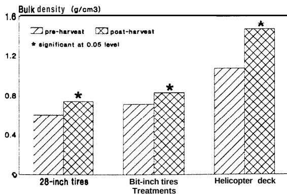
Figure 2. Soil bulk density by treatment.
