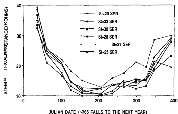
Figure 1. Monthly stem electrical resistance (K ohm) readings on loblolly pine trees from stands of varying site indices.
