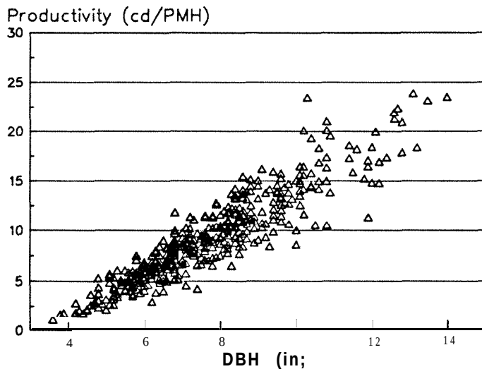
Figure 2. Calculated productivity for the 435 observations for the Norcar 600 H harvester.
