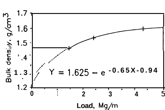
Figure 1. Effect of the different compactor loads on the bulk density in the 0 to 10 cm depth.
