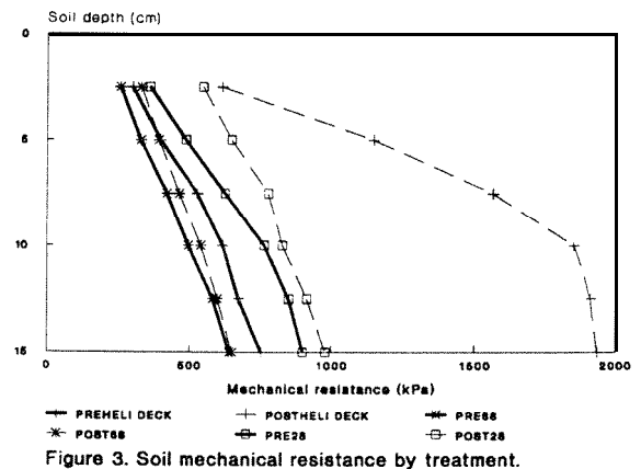
Figure 3. Soil mechanical resistance by treatment.
