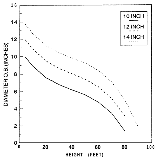
Figure 3. Stem taper of mean diameter classes in 50-year-old loblolly pine thinning treatments in the SC Piedmont.
