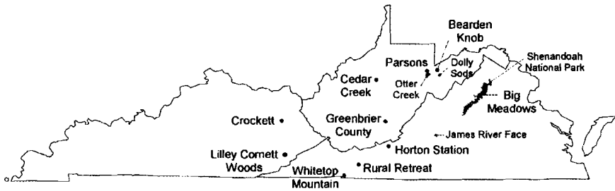
Figure 1. Locations of the ozone monitoring sites (solid black dots) and Class I Wildernesses (grey shaded areas).
