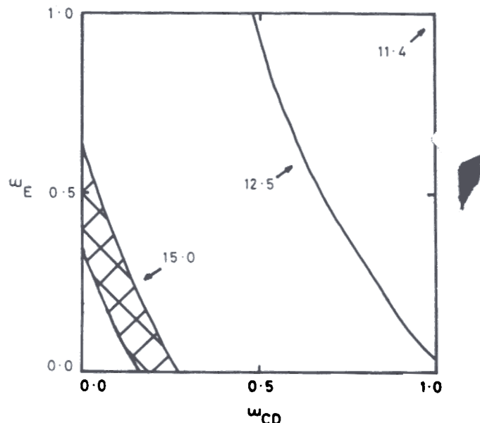
Figure 5. Mean square dipole moment as functions of \omega_E and \omega_{CD} . A contour line is drawn at 12.5. The maximum squared dipole moment is 16.9 D 2 at \omega_E = \omega_{CD} = 0 . At the opposite corner, where \omega_E = \omega_{CD} = 1 , \langle \mu^2 \rangle is 11.4 D 2 . The experimental result at 300 K, \langle \mu^2 \rangle^{1/2} = 3.91 \pm 0.04 D, is denoted by the cross-hatched region
