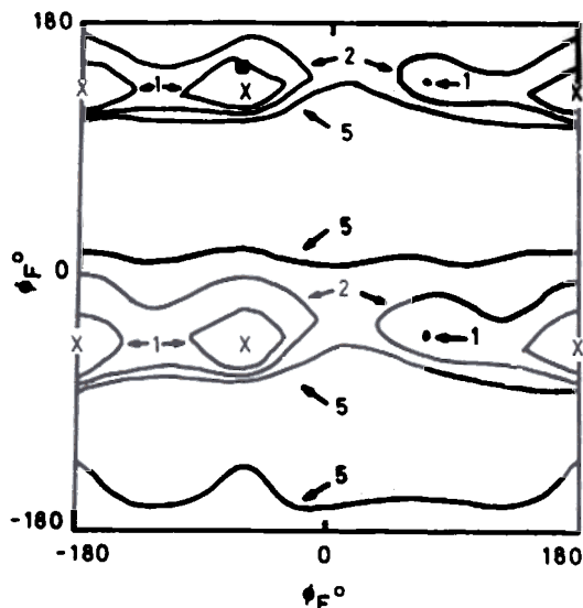
Figure 4. Conformational energy surface for rotations about the C(3)-O(2) ( \phi_E ) and C(2)-C(11) ( \phi_F ) bonds. Essentially identical minima occur at positions denoted by X. Contours are drawn at energies 1, 2, and 5 kcal mol -1 above the minima. The square denotes the conformation found in crystalline (-)-epicatechin
