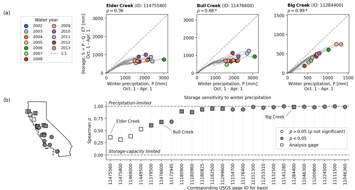
Figure 1. Method of determining the dependence of subsurface winter storage ( S ) on winter precipitation ( P ) across select undisturbed Californian basins. (a) For each water year, S is calculated as the remainder of the catchment mass-balance and plotted as a function of cumulative winter precipitation (October 1st to April 1st). The gray lines show the seasonal progression of S (calculated daily). Early wet season rainfall primarily increases S , generating minimal streamflow. In basins where subsurface storage is more likely to be annually refilled (where S plateaus), further P does contribute to streamflow, resulting in a curved line. If all precipitation went into storage without drainage to groundwater or evapotranspiration, catchments would plot along the dashed 1:1 line. The Spearman rank correlation coefficient ( \rho ) is calculated for each watershed; asterisks denote significance at p < 0.05 . (b) Spearman rank correlations across basins and location of basins in the greater state of California. Filled symbols denote significance at p < 0.05 . Those watersheds where wet season precipitation exceeds dry season accrued vadose zone storage deficits for at least 5 years over a 20 years analysis period (2000–2020) highlighted with square markers. Calculation of \rho restricted to 2002–2013 water years to match the original Hahm et al. (2019) data set and minimize non-stationary conditions introduced by mass tree mortality at the end of the period (USDA, 2016). We diverge from Hahm et al. (2019) in using actual, instead of potential, evapotranspiration in our calculation of S . Plotting space based on Figures 2 and 3 of Hahm et al. (2019).
