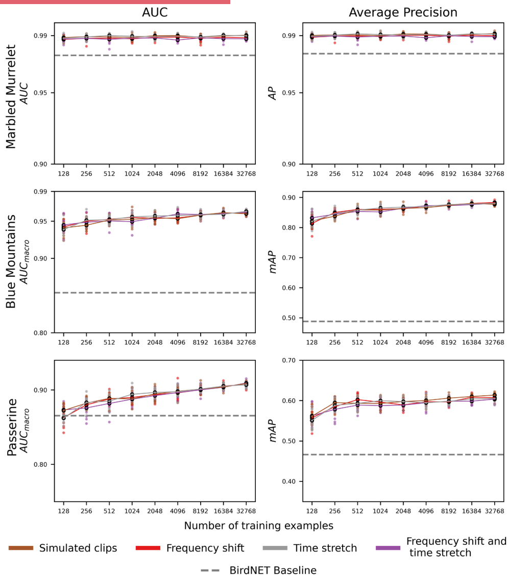
FIGURE 3 Relative effects of increasing the number of simulated clips and three acoustic data augmentation techniques relative to soundscape simulation without acoustic augmentations for acoustic classification algorithms using transfer learning under data scarcity. Increasing the number of simulated soundscapes consistently improved relative model performance, with no evidence of overfitting. The number of simulated examples varied, and the dataset construction and training were replicated 10 times. Dark points and lines indicate the average performance of the acoustic augmentations.
