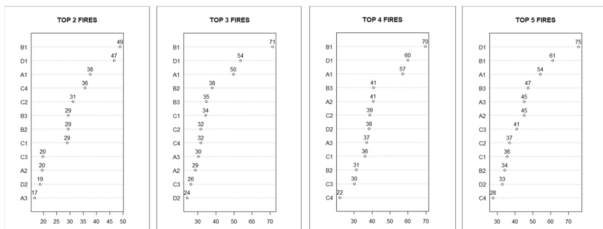
Fig. 9. Mean Decrease Accuracy (MDA) reported for different Random Forest models.
