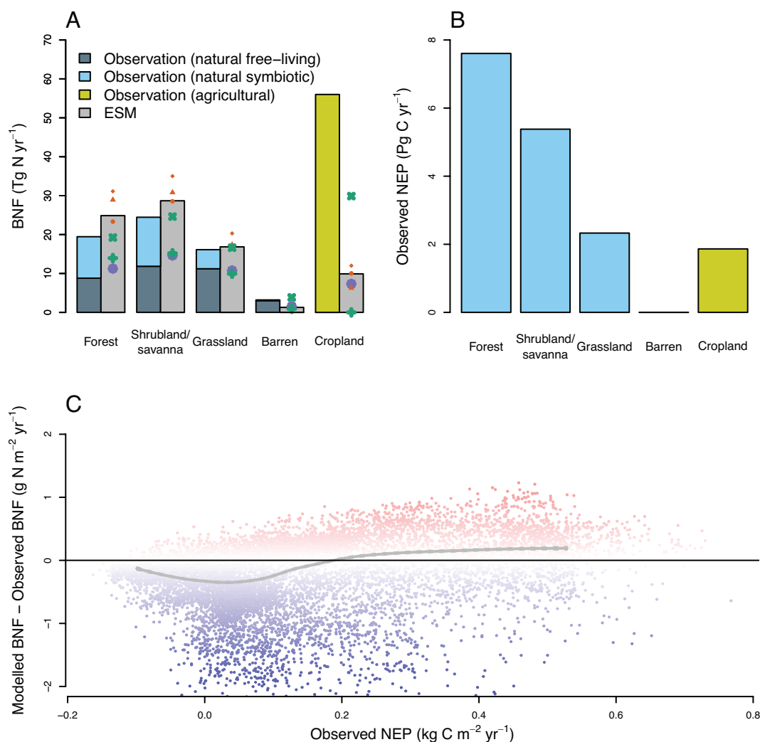
Fig. 3. Comparison between empirical and modeled present-day terrestrial BNF across biomes relative to NEP. ( A ) Empirical and modeled BNF (median and interquartile range) across International Geosphere–Biosphere Programme (IGBP) biomes (35), where empirical BNF is separated into free-living BNF and symbiotic BNF. Each point represents the average of ESMs with the same land surface model, and colors and shapes match Fig. 1. ( B ) Empirical NEP across IGBP biomes from ref. 36. ( C ) Discrepancy between empirical BNF and modeled BNF over NEP, where blue areas indicate underestimation by ESMs and red areas indicate overestimation by ESMs relative to observations. Each point is a grid cell.
