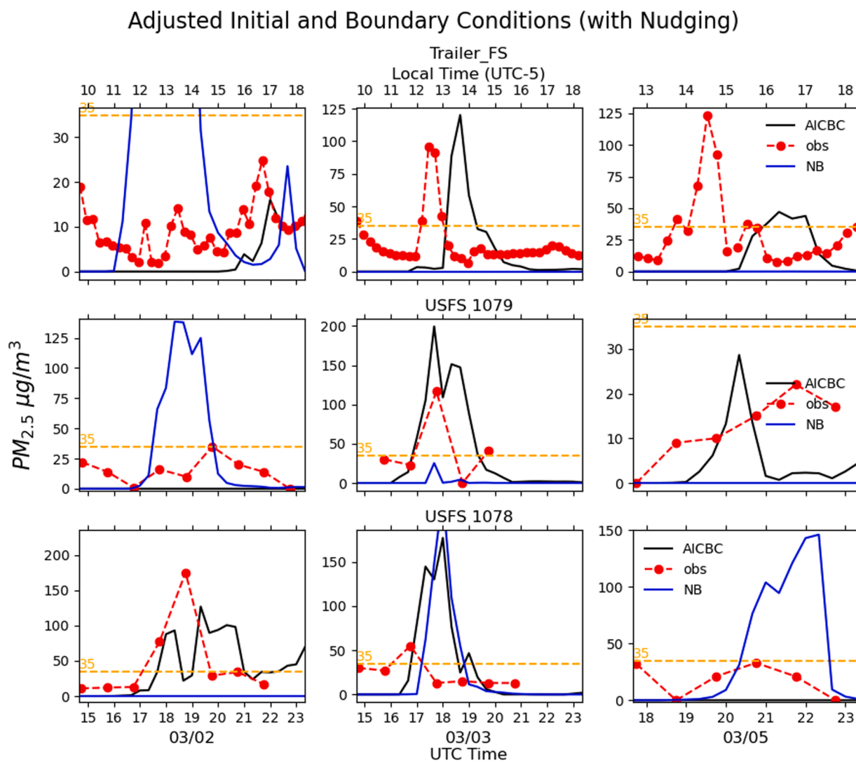
Fig. 4. Observed and simulated PM_{2.5} concentration (AICBC with nudging) at Traylor FS (TEOM), USFS 1079 (EBAM), and USFS 1078 (EBAM) monitors on three prescribed fire days. The red dots with the dashed line, blue solid line, and black solid line indicate the observation, NB simulation, and AICBC simulation, respectively. The orange dashed line marks the 35 \mu g/m^3 PM_{2.5} level, which is the daily standard in the U.S. (Agency, U.E.P 2012).
