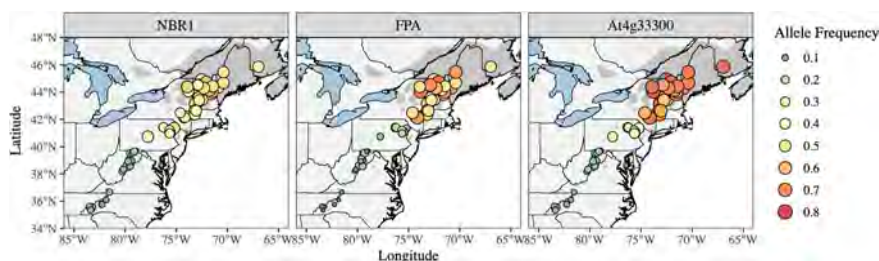
Fig. 7.8 Among-population variation in red spruce ( Picea rubens ) climate-adaptive alleles for three candidate genes identified through gene-environment association analysis. Figure used with permission of John Wiley & Sons, from Capblancq et al. (2022); permission conveyed through Copyright Clearance Center, Inc.
