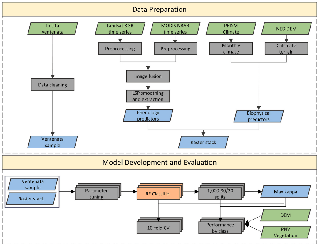
Fig. 1. The framework applied to investigate the detection and mapping of ventenata populations.
