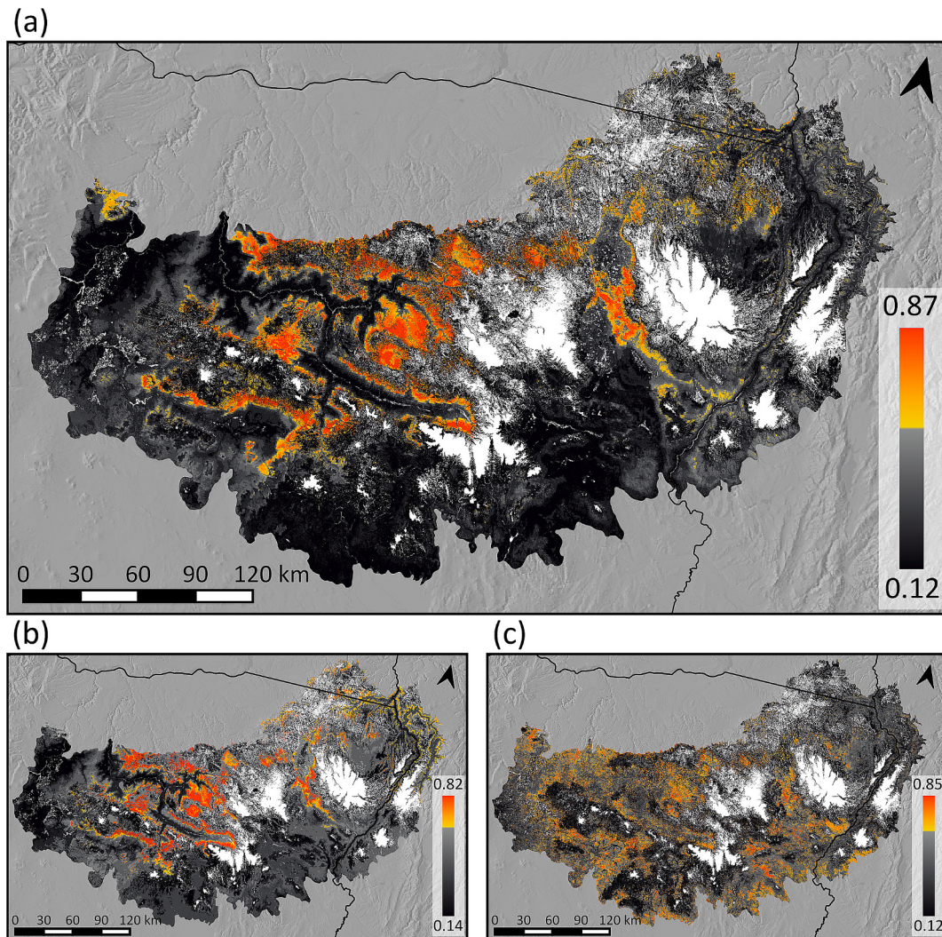
Fig. 5. Predictions from a) the hybrid model, b) the bioclimatic model, and c) the phenology model. The color ramp is split at the threshold that maximizes kappa (hybrid = 0.58, bioclimatic = 0.73, phenology = 0.7), where areas above the threshold (heavily invaded) are yellow to red and areas below the threshold are grey to black. Masked areas (white) are presumed to be currently uninhabitable due to high elevation, high forest canopy cover, or perennial water. (For interpretation of the references to colour in this figure legend, the reader is referred to the web version of this article.)
