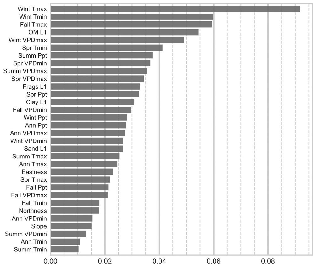
Fig. A2. Variable importance and rank of the 32 predictors in the bioclimatic model.
