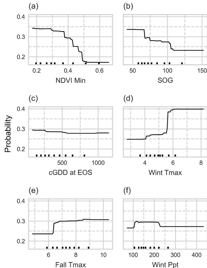
Fig. 4. The relationship between the probability of heavily invaded areas and the top predictors from the hybrid model. Tick marks in the rug plot along the x-axis indicate deciles. Predictors include a) minimum NDVI (NDVI), b) start-of-green-up (day-of-year), c) cumulative growing degree days at the end-of-season ( ^{\circ}\text{C} ), d) average winter maximum temperature ( ^{\circ}\text{C} ), e) average fall maximum temperature ( ^{\circ}\text{C} ), and f) average total winter precipitation (mm). (For interpretation of the references to colour in this figure legend, the reader is referred to the web version of this article.)
