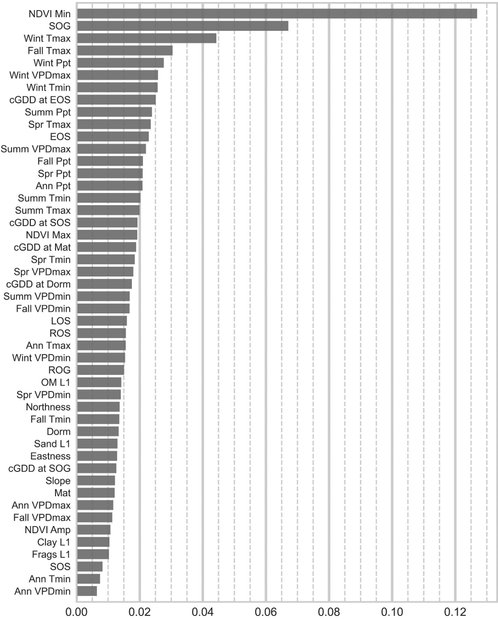
Fig. A1. Importance and rank of the predictors included in the hybrid model.
