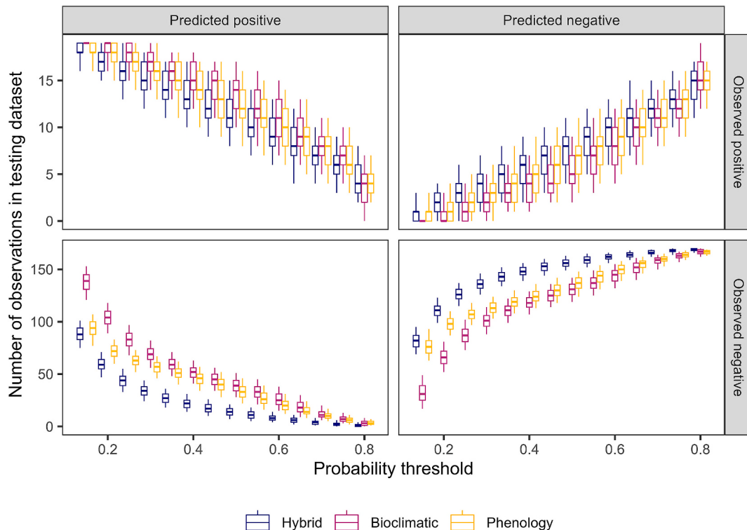
Fig. 3. Confusion matrix showing the distribution of predicted vs. observed positive and negative classes in the three models. The positive class represents ventenata populations of 20 % or greater cover and the negative class represents populations with less than 20 % cover. The upper and lower bounds of each box plot show the 25th and 75th quantiles, the whiskers show the 5th and 95th quantiles, and the mid line shows the median.
