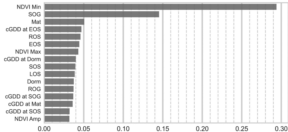
Fig. A3. Variable importance and rank of the 16 predictors in the phenology model.
