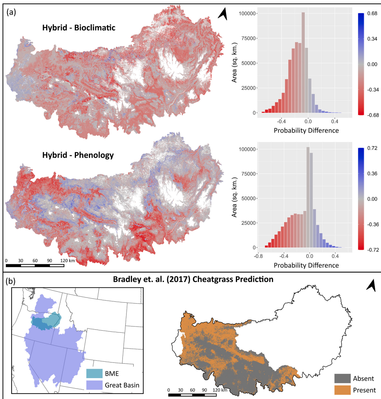
Fig. 7. Ventenata model differences and cheatgrass predictions where a) shows the difference in ventenata model predictions and b) shows predicted as cheatgrass (> 15 % cover) within a subset of the BME (Bradley et al., 2017). In panel a, blue indicates that the hybrid model predicted a higher probability, while red indicates that the bioclimatic or phenology model predicted a higher probability. (For interpretation of the references to colour in this figure legend, the reader is referred to the web version of this article.)
