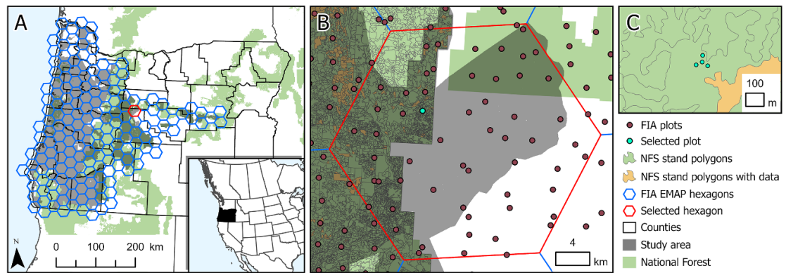
Figure 1. (A) Study area in Oregon, USA, consisting of a patchwork of 20 airborne LiDAR collections, which matches the study area of Mauro et al (2021b), the smallest common area across the 10 aboveground biomass density (AGBD) map products compared. (B) The FIA EMAP hexagon selected for illustration purposes; the publicly available FIA plot locations shown are perturbed; i.e. not the accurate but confidential plot locations used in the analysis. (C) The FIA plot selected for illustration purposes; each FIA plot has this same configuration of 4 subplots. FIA plots have no relationship to NFS stands. EMAP: Environmental Monitoring and Assessment Program; FIA: Forest Inventory and Analysis; NFS: National Forest System.
