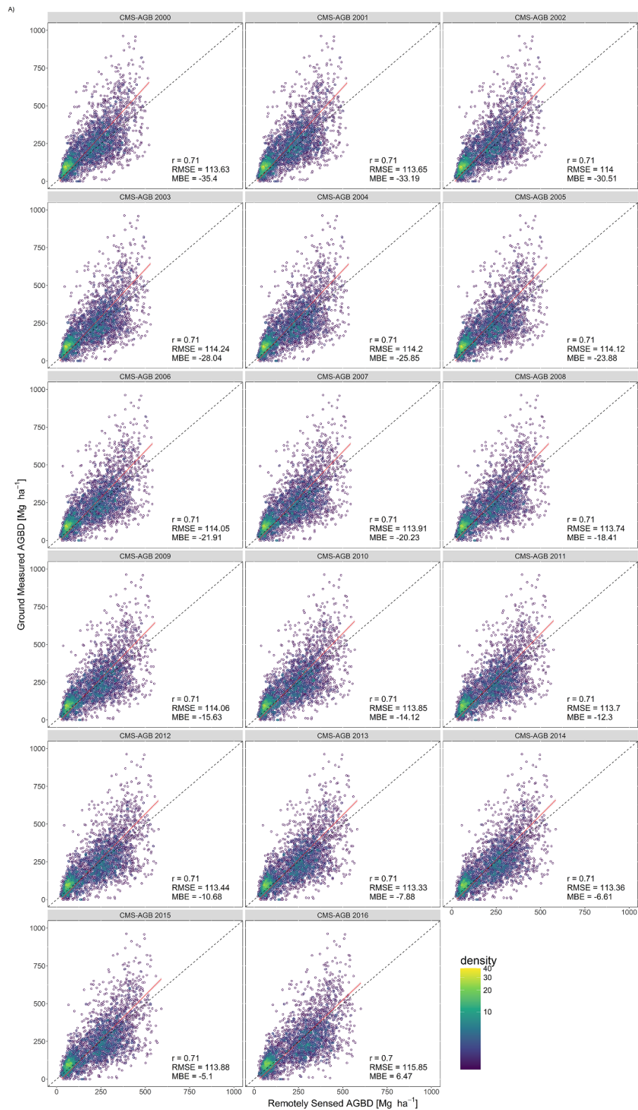
Figure 3. Ground-based AGBD observations regressed on mean AGBD estimates from (A) CMS-AGB and (B) GNN maps after aggregation at the stand level. The pink shaded area around the red solid line of best fit represents the 95% confidence interval. AGBD: aboveground biomass density.
