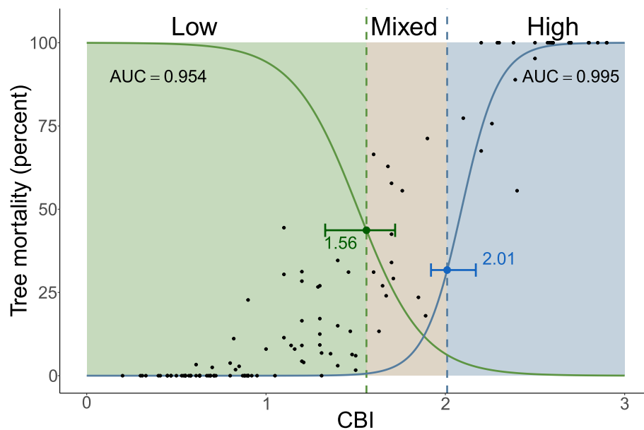
Fig. 3 Relationship between percent tree mortality (y-axis) and CBI (x-axis) from Parks et al. (2023). LANDFIRE classes low severity as <25% tree mortality, mixed severity as between 25 and 75%, and high severity as >75%. We show the median logistic regression curves with thresholds for low to mixed ( T_{lm} ) and mixed to high ( T_{mh} ) marked by vertical dashed lines, and we show the median threshold with 95% bootstrapped confidence intervals with colored points and error bars. Median and 95% confidence intervals for T_{lm} and T_{mh} are 1.56[1.33, 1.72] and 2.01[1.92, 2.17], respectively. AUC is the mean bootstrapped AUC. Additional accuracy statistics are in Appendix B
