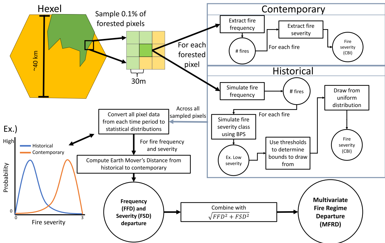
Fig. 2 Workflow of our analysis within a single landscape polygon. Circles represent numeric outputs while rectangles are operations. We sampled forested pixels (in green) and performed the operations in the light blue box for each pixel. Then, we converted those results to normalized distributions of fire frequency and severity for historical and contemporary time periods. From these distributions, we calculated EMD between historical and contemporary fire frequency departure (FFD) and fire severity departure (FSD), which are combined into a multivariate fire regime departure (MFRD) index. This analysis is replicated 100 times for each landscape, and our primary summaries are the median FFD, FSD, and MFRD
