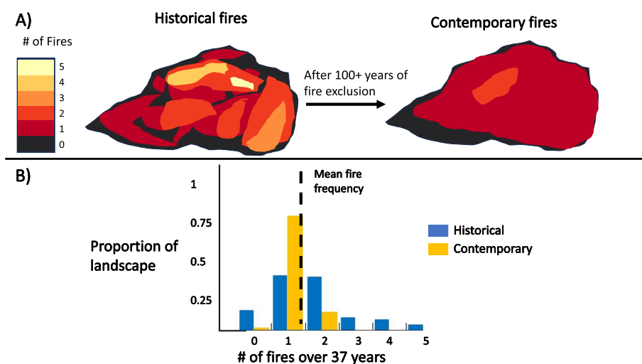
Fig. 1 Conceptual diagram of fire regime change in a historically frequent fire ecosystem when observed over 37-year historical and contemporary periods. A Transitioning from a frequent fire system to an infrequent fire system due to fire exclusion leads to homogenization in spatial patterns of fire occurrence. B As a result, the statistical distributions of fire frequency during historical and contemporary periods are different. However, the contemporary and historical periods have the same mean fire frequency, marked by the dashed line. Means do not characterize the homogenization of the fire frequency distribution through time
