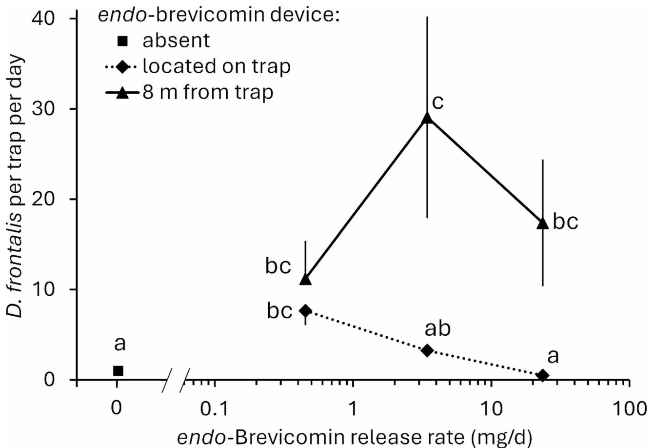
Fig. 4 Experiment 2: Response of D. frontalis to widely spaced, single funnel traps baited with an invariable release rate of frontalinal and turpentine plus a variable release rate of endo -brevicomin from a device located either on or 8 m from the trap. Error bars display standard
