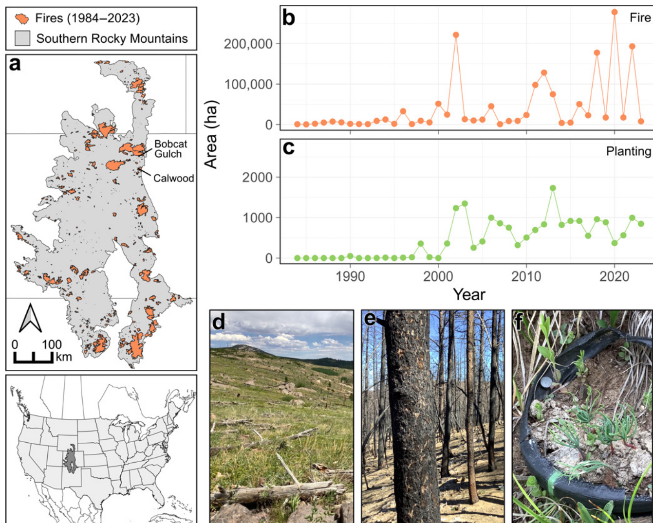
FIGURE 1 (a) The study area (including fire perimeters between 1984 and 2023) in the Southern Rocky Mountains, USA, (b) the annual area burned by wildfire (c), post-fire tree planting activities on USDA Forest Service lands, (d, e) characteristics of the two locations of experimental field trials of direct tree seeding, and (f) a depiction of our direct seeding field trials. (d) The Bobcat Gulch sites burned in 2000 and (e) the Calwood sites burned in 2020; photos (d, e) were taken ca. 2021. Photo credit: C. Schloegel.
