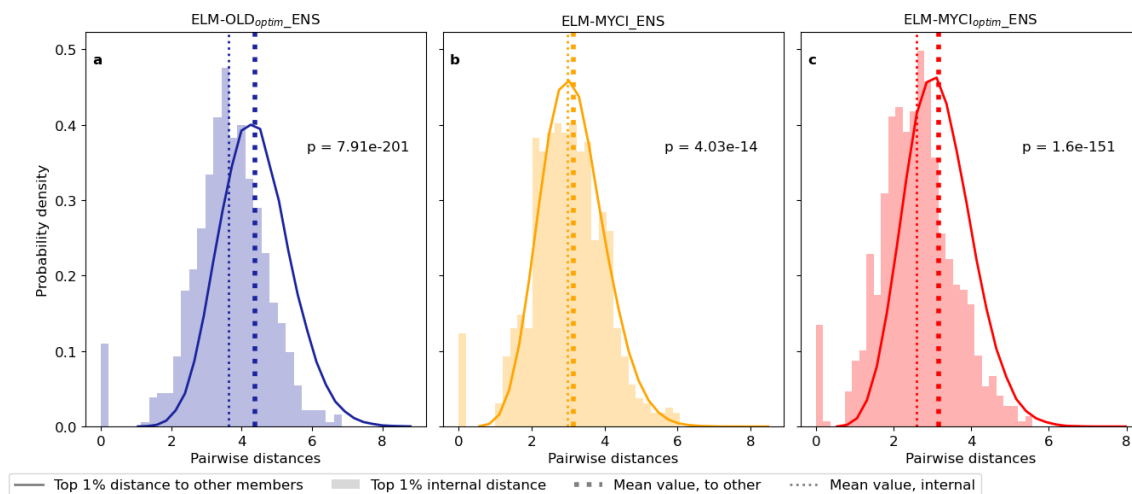
Figure 9. Probability density distributions of the Euclidean distances between the parameter values of two groups of pairs of ensemble members: between the best-performing 1 % members (shaded bars), and between the best-performing 1 % members and the other 99 % members (solid line). Displayed probability densities are pooled from all pairs in each group. The p -values in each panel indicate whether the two groups are significantly different, using two-sided t -test for the mean values of two independent samples.
