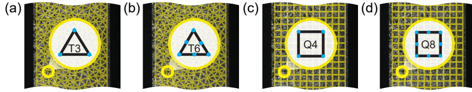
Figure D.5: Examples of global DIC element shape functions: (a) linear triangle, (b) quadratic triangle, (c) quasi-linear quadrangle, and (d) quadratic quadrangle
