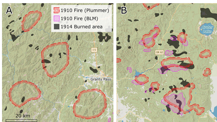
Figure 4. A) 1910 fires mapped by Plummer (1912) that were recorded as unburned in the 1914 survey (Elliott and Rowland 1914). B) 1910 fires mapped by Plummer (1912) compared to those compiled by the Bureau of Land Management (BLM 2020), illustrating disagreements in the size and location of individual fires. The BLM dataset contained only a small number of 1910 fire perimeters, compiled from an unknown source. While Plummer (1912) offered the most complete and well-documented record of the 1910 fires, our impression is that the size of the perimeters was substantially overestimated.
