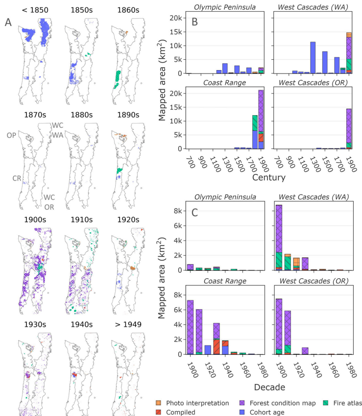
Figure 1. A) Mapped fire perimeters and burned areas across forested westside ecoregions up to 1984, color-coded by the original source type. For each ecoregion/state, areas are tabulated by B) century and C) decade. The Olympic Peninsula (OP), Coast Range (CR), Western Cascades of Washington (WC WA), and Western Cascades of Oregon (WC OR) are outlined in grey and labeled in panel A. Note that the database does not represent a spatially or temporally complete sample and should not be used to directly interpret trends in area burned.
