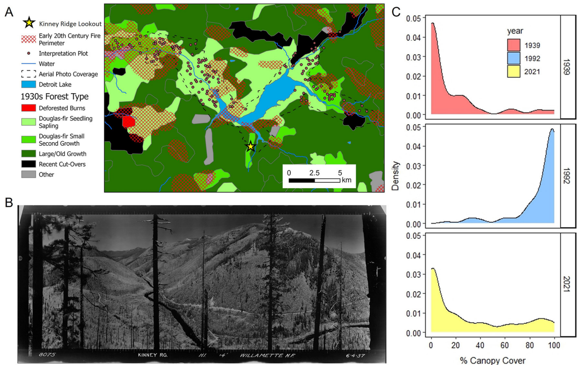
Figure 5. A) The case study area around the North Santiam River (central Oregon) with the location of photo-interpreted plots, forest conditions in the 1930s (Harrington 2003), and early 20 th century burned areas (Thompson and Johnson 1900). B) The view from the fire lookout on Kinney Ridge (yellow star on panel A) in 1937 looking northwest down the North Santiam River. C) The probability density of photo-interpreted canopy cover at plot locations in 1939, 1992, and 2021 across the area covered by available 1939 aerial photos.
