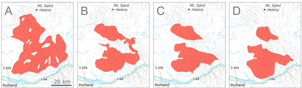
Figure 2. Conflicting perimeters for the 1902 Yacolt Burn (southwestern WA) from A) Cox (1902; fire atlas), B) and C) Gifford Pinchot (GP dataset; fire atlas), and D) Wildland Fire Decision Support System (2018; compiled). We ultimately included the Cox perimeter because it was published in a contemporary report with documentation, while the primary sources of the other datasets were unknown.
