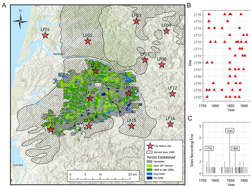
Figure 6. A) Map of burned areas (Thompson and Johnson 1900) near the Elliott State Forest (ESF; coastal Oregon) and the location of fire history sites used to reconstruct historical fires. Age structure on the ESF (West and Strimbu 2024) is illustrated by color and demonstrates the spatial variability in stand establishment years within the forest. B) Records of historical fires at fire history sites on the ESF. Red triangles indicate the precise year of historical fires. C) The number of fire history sites recording fires from 1750–1910. Fires in 1776, 1849, and 1868 were extensive, but most historical fires were only evidenced at 1–2 sites. Fire history and age structure at the ESF illustrate that maps and written descriptions of historical fires may describe the effects of multiple fires in the preceding decades.
