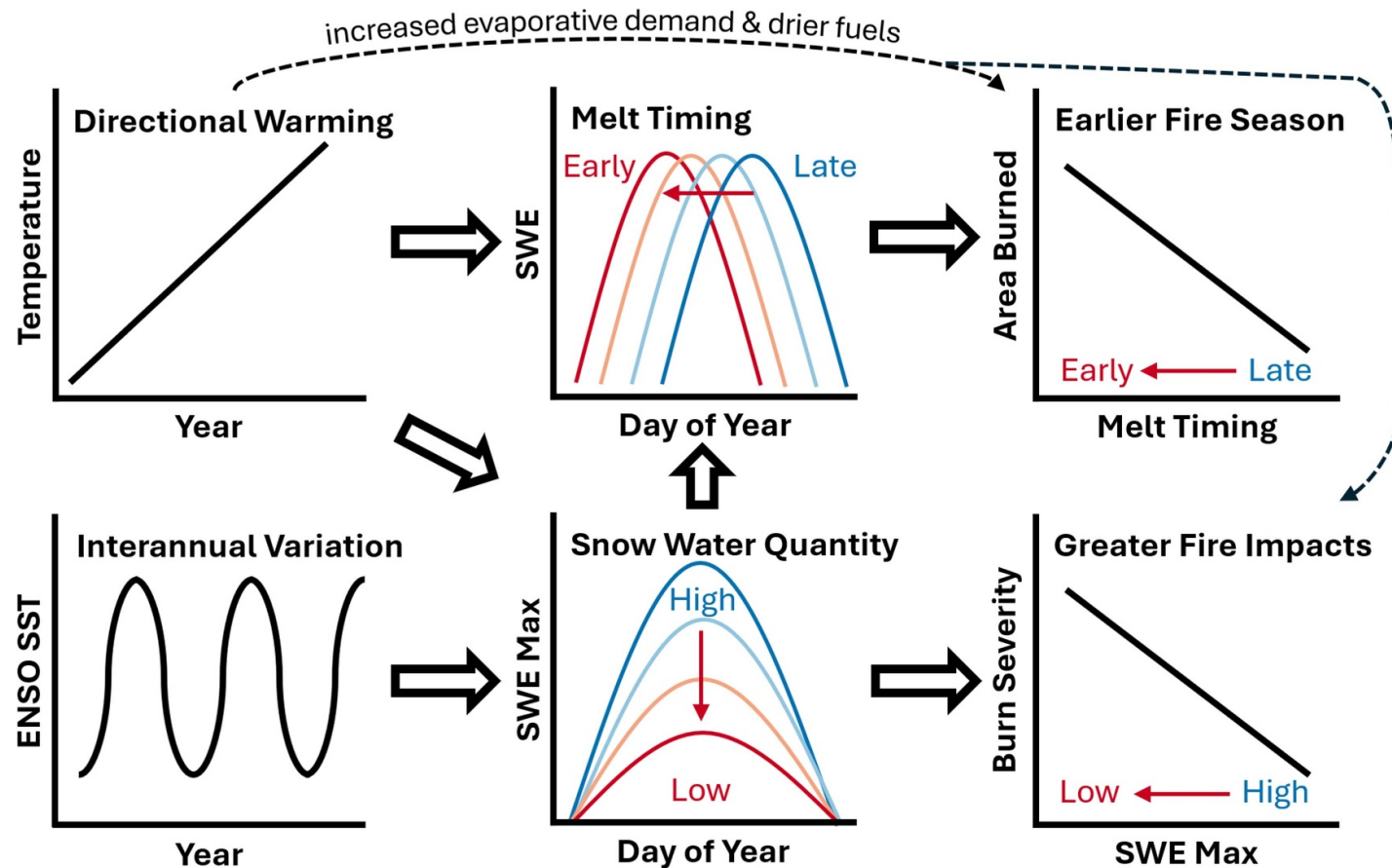
Figure 5. Climate warming, snowpack decline, and growing forest fire impacts to snow-dominated western US watersheds. Climate warming reduces snowpack and advances snowmelt timing, which is associated with longer fire seasons and greater area burned. Climate warming can also increase area burned and burn severity independent of effects on snowpack, through mechanisms not studied here, represented by dashed lines. Interannual variability in snowpack water quantity influences fire severity, with long-term decline and low SWE conditions associated with more severe burn outcomes that may promote increased tree mortality and altered watershed hydrologic function.
