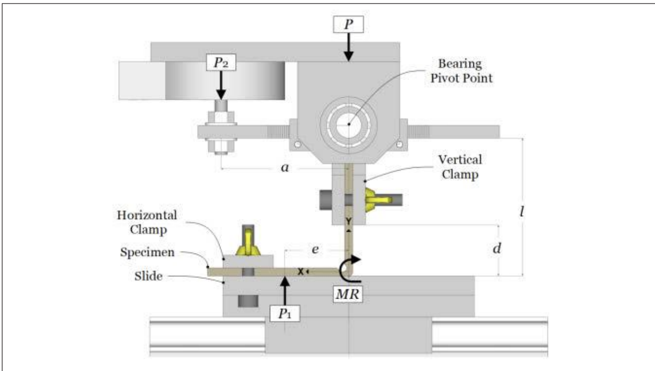
5. Diagram of the eccentricity ( e ) fixture. Eccentricity is measured from the center of the board to the interior of the box. The extent of e is exaggerated for visualization; more typically, the eccentricity falls within the thickness of the board specimen, especially near failure ( MR : residual moment).
