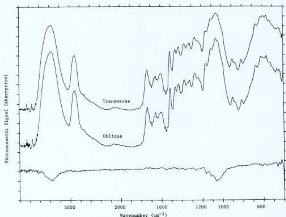
FIG. 4. Comparison of FTIR-PAS spectra of ponderosa pine transverse (top) and oblique ( 45^\circ to the longitudinal direction, middle) sections. The lower spectrum is the difference between the transverse and oblique spectra.
