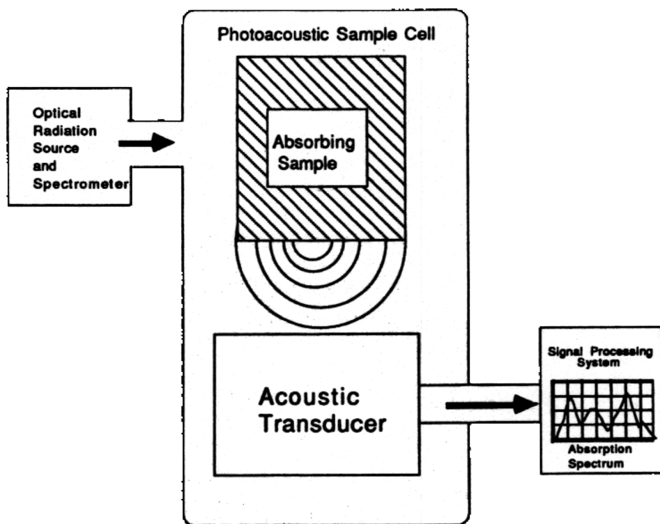
FIG. 1. Schematic of the photoacoustic spectroscopy technique (reproduced with permission from McClelland 1982).
