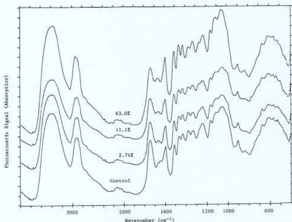
FIG. 5. FTIR-PAS spectra of eastern cottonwood samples with various degrees of decay by the brown-rot fungus Gleophyllum trabeum . Numbers labelled on each spectrum represent average percentage weight loss of the sample due to decay.
