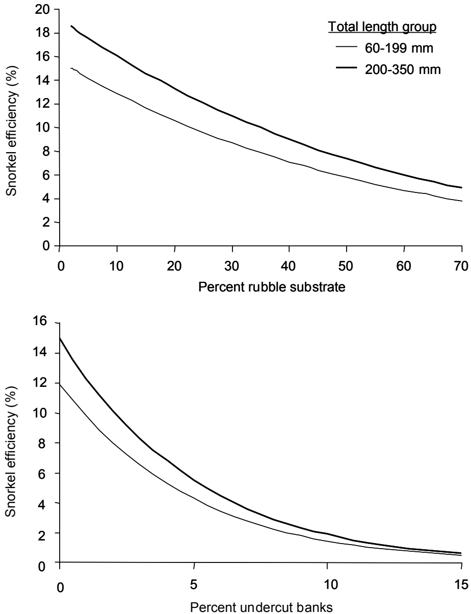
Figure 3. Predicted day snorkeling efficiency for two total length size classes of bull trout versus percent rubble substrate (top) and percent undercut banks (bottom). Predictions based on best fitting beta binomial model and assuming 1.6% percent undercut banks (top) and 30% rubble substrate (bottom).
