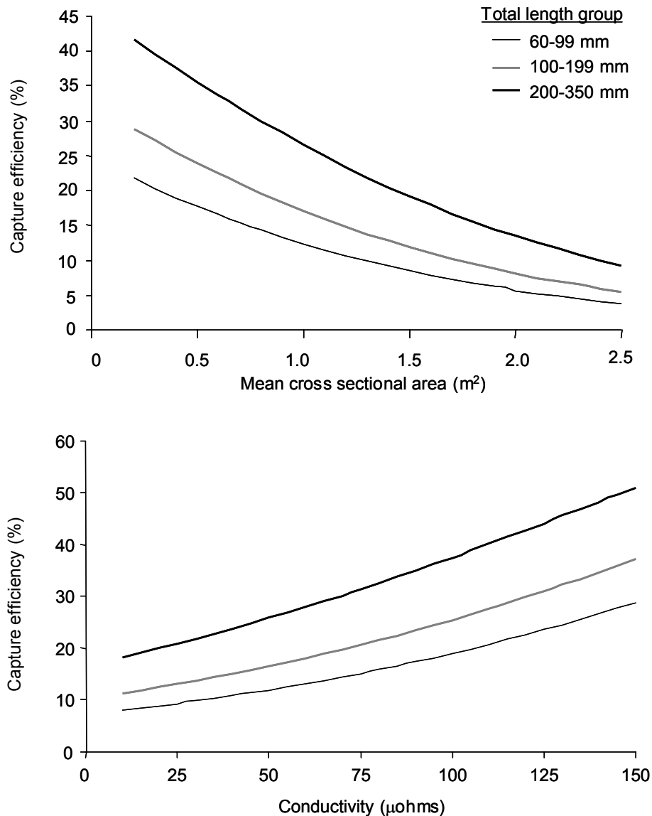
Figure 7. Predicted single-pass electrofishing capture efficiencies for three total length size classes of bull trout versus stream cross-sectional area (top) and conductivity (bottom). Predictions based on best fitting best-fitting beta binomial model and assuming conductivity of 54 (top) and 1 m 2 cross-sectional area (bottom).
