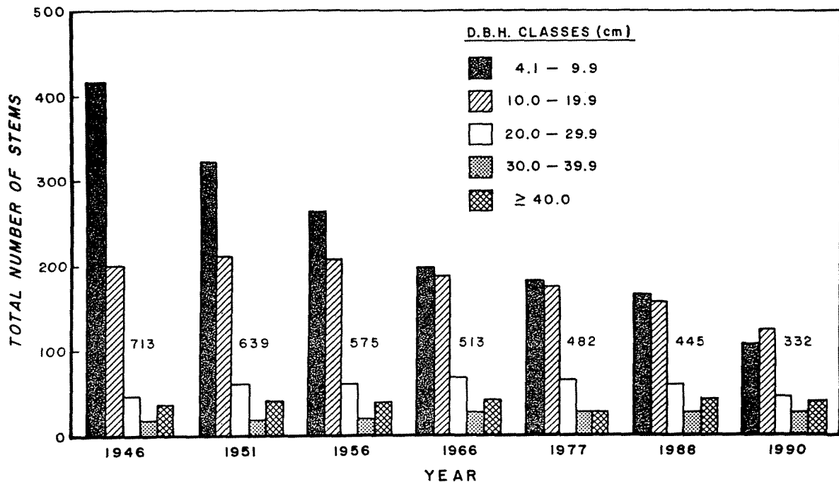
Figure 15.—Diameter class distributions in 7 different years on long-term plot TR-1 in the Baño de Oro Natural Area. The numbers in the declining sequence from 713 to 332 refer to total stems in the plot.
