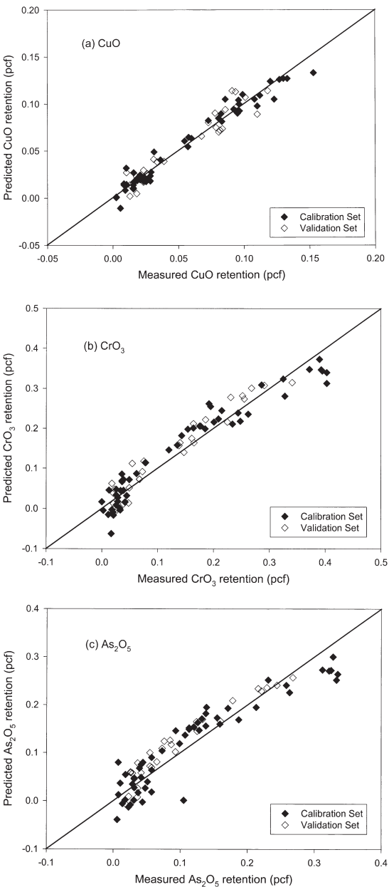
FIG. 5. Relationship between measured values of: (a) CuO, (b) CrO 3 , and (c) As 2 O 5 retentions and those predicted by PLS-2 modeling using NIR spectra for CCA samples.
