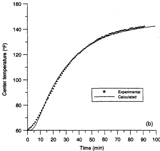
FIG. 5. Experimental and calculated increase in center temperature of slash pine with time while heated at 160°F (71°C) dry bulb: (a) 1.0-in.- (25-mm-) thick, 50°F (2.8°C) wet bulb depression; (b) 1.8-in.- (46-mm-) thick 15.7°F (8.7°C) wet bulb depression. [ ^{\circ}\text{C} (temperature) = (^{\circ}\text{F} - 32)/1.8 ; ^{\circ}\text{C} (wbd) = ^{\circ}\text{F}/1.8 ]
