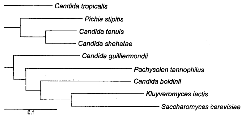
Fig. 2. Phylogenetic tree of XRs or ARs found in yeasts. Amino acid sequences were identified by BLAST, and the resulting protein sequences were then aligned. A phylogenetic tree was generated from the aligned regions after excluding sequences creating gaps.
