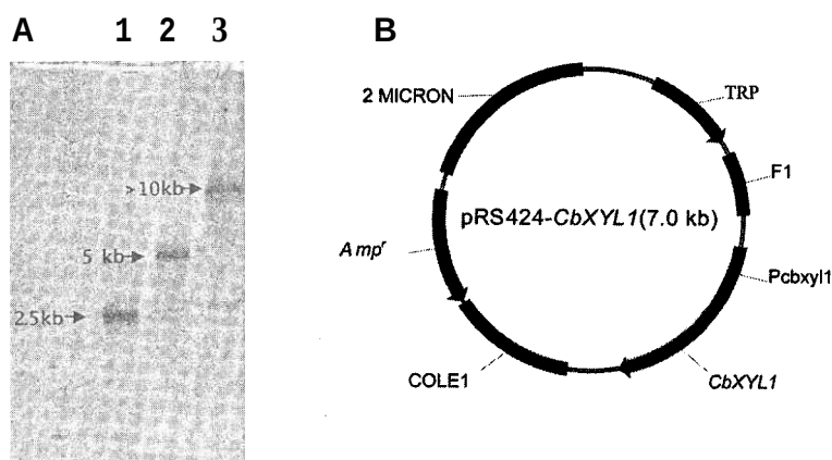
Fig. 3. Genomic Southern blot analysis of CbXYL1 and construction map for expression in S. Cerevisiae . (A) Genomic DNA from C. boidinii was digested with Msc I, Pst I, and Xba I. After running on an agarose gel, DNA was transferred onto a nylon membrane, hybridized with probe DNA that was synthesized by random primer extension. The signal was then developed according to a protocol given by Roche. Arrows indicate the approx size of hybridized DNA fragments. (B) Construction map of pRS424- CbXYL1 for expression in S. cerevisiae . The CbXYL1 gene was constructed under the control of its own promoter. PRS424- CbXYL1 was introduced into S. cerevisiae L2612 (Mata, trp - , ura - , leu - ) (12). Pcbxyl1 and CbXYL1 indicate promoter and coding region, respectively.
